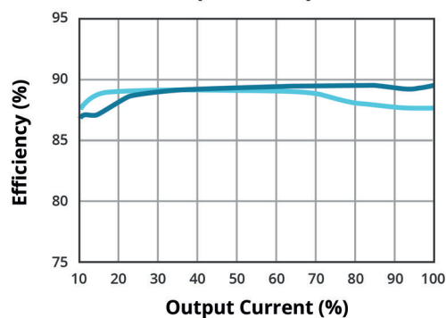
EFFICIENCY VS OUTPUT LOAD (PSK-36E-5)
