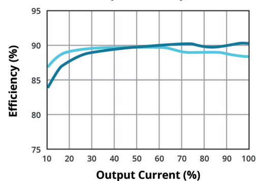
EFFICIENCY VS OUTPUT LOAD (PSK-36E-12)
