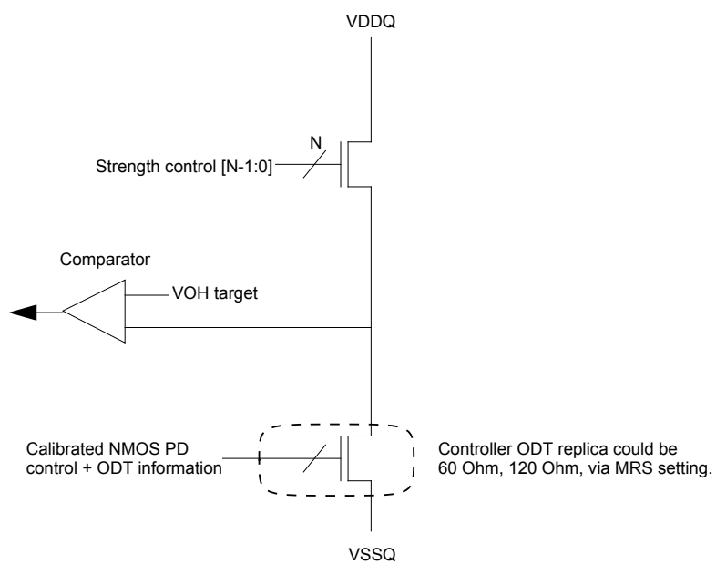
Figure 22. pull-up calibration
