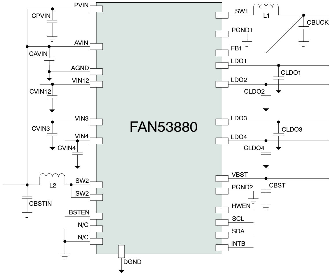
Figure 1. Application Diagram
