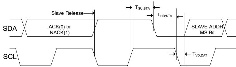
Figure 33. REPEATED START Condition
