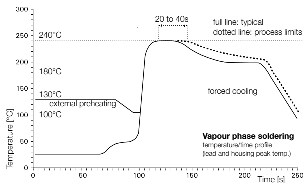
Recommended vapor phase soldering profile
