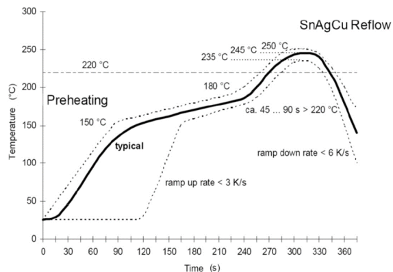
Recommended reflow soldering profile IEC 61760-1
