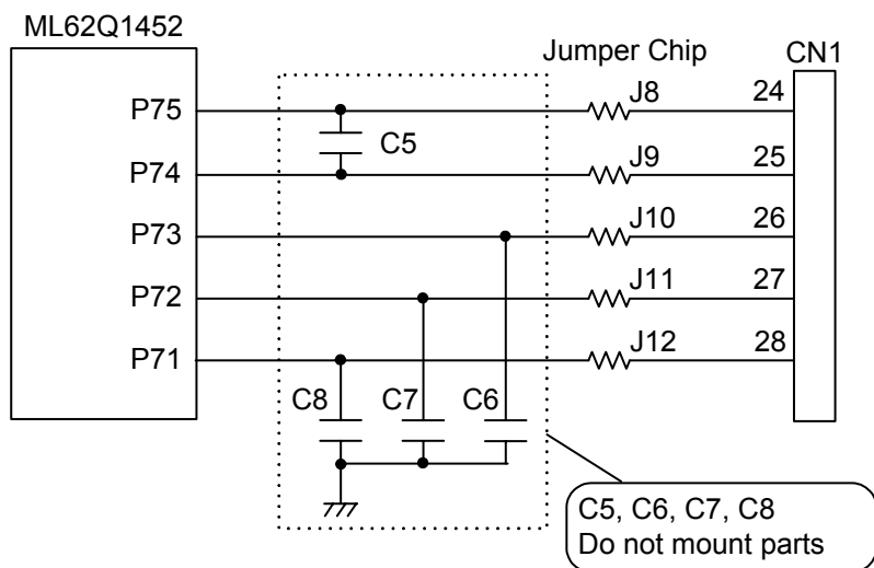
Fig.6 P75 - P71 Circuit
