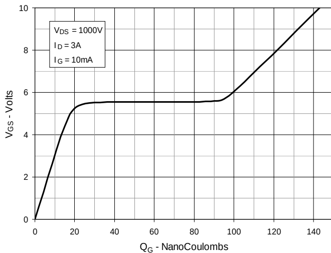
Fig. 9. Gate Charge
