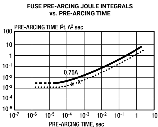
Fig. 5b. Choice of fuse, example #5
