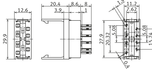
External dimensions
