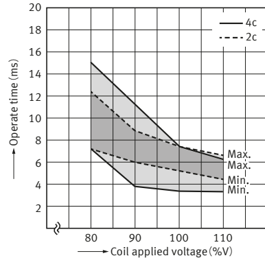
4. Operate time
