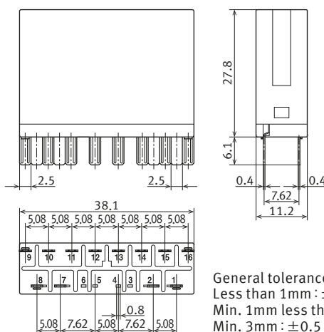
External dimensions
