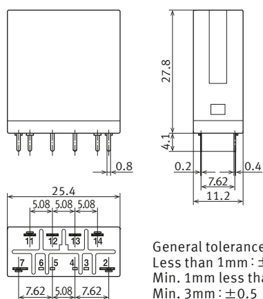
External dimensions
