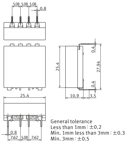
External dimensions
