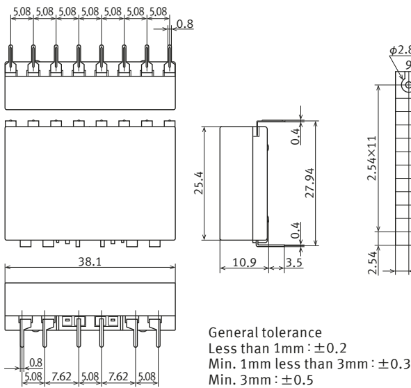
External dimensions
