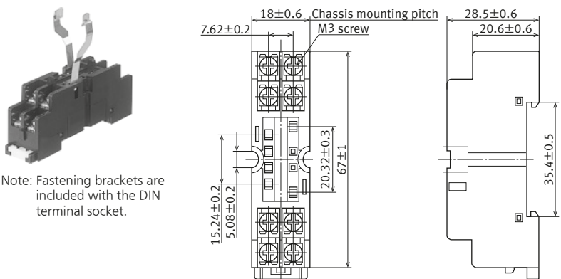
External dimensions
