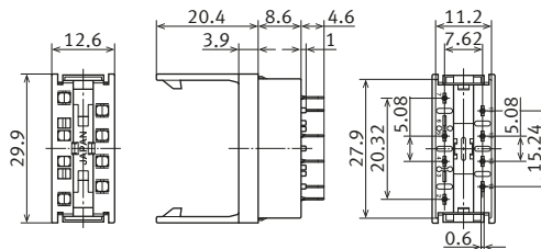
External dimensions
