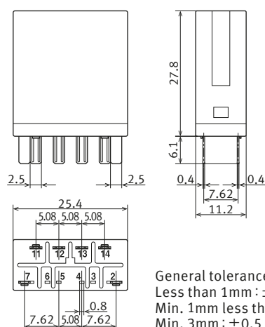
External dimensions
