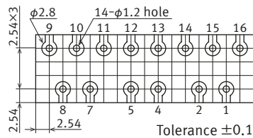
Recommended PC board pattern ( BOTTOM VIEW )
