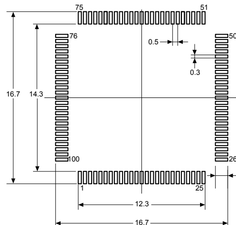
Figure 49. LQFP100 - Footprint example
