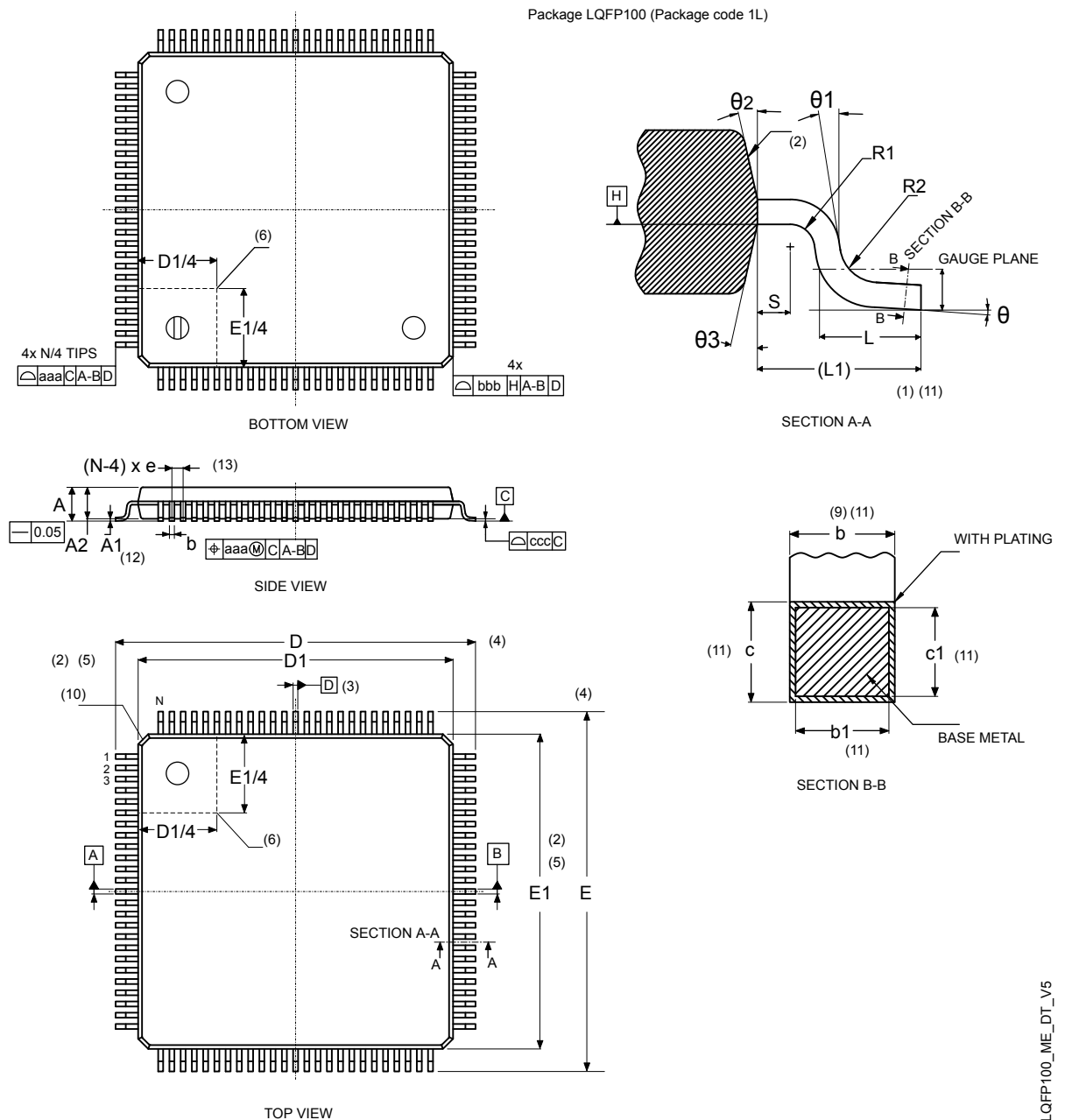
Figure 48. LQFP100 - Outline (15.)
