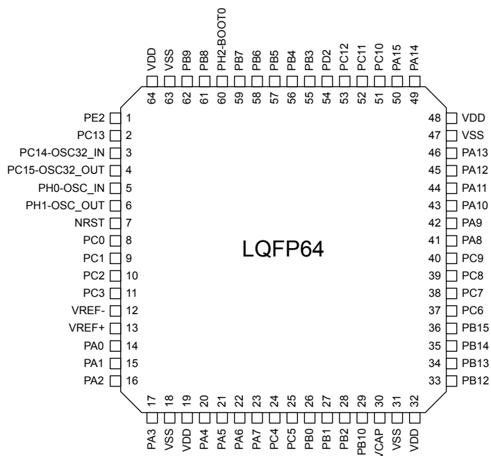
Figure 8. LQFP64 alternative pinout
