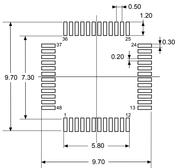
Figure 42. LQFP48 - Footprint example
