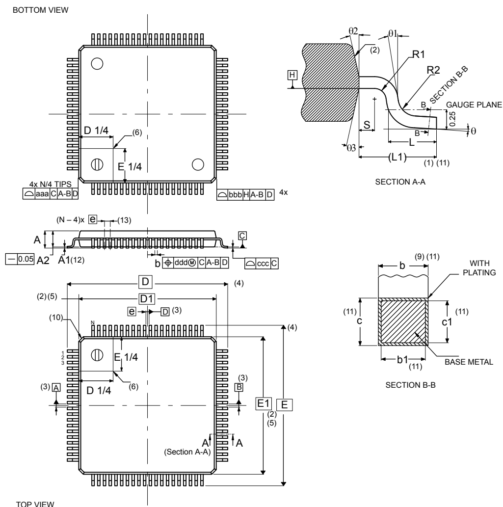
Figure 46. LQFP80 - Outline (15.)
