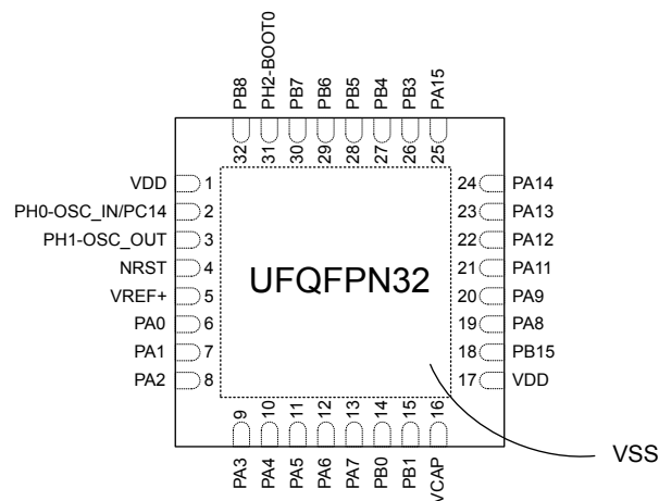
Figure 4. UFQFPN32 pinout
