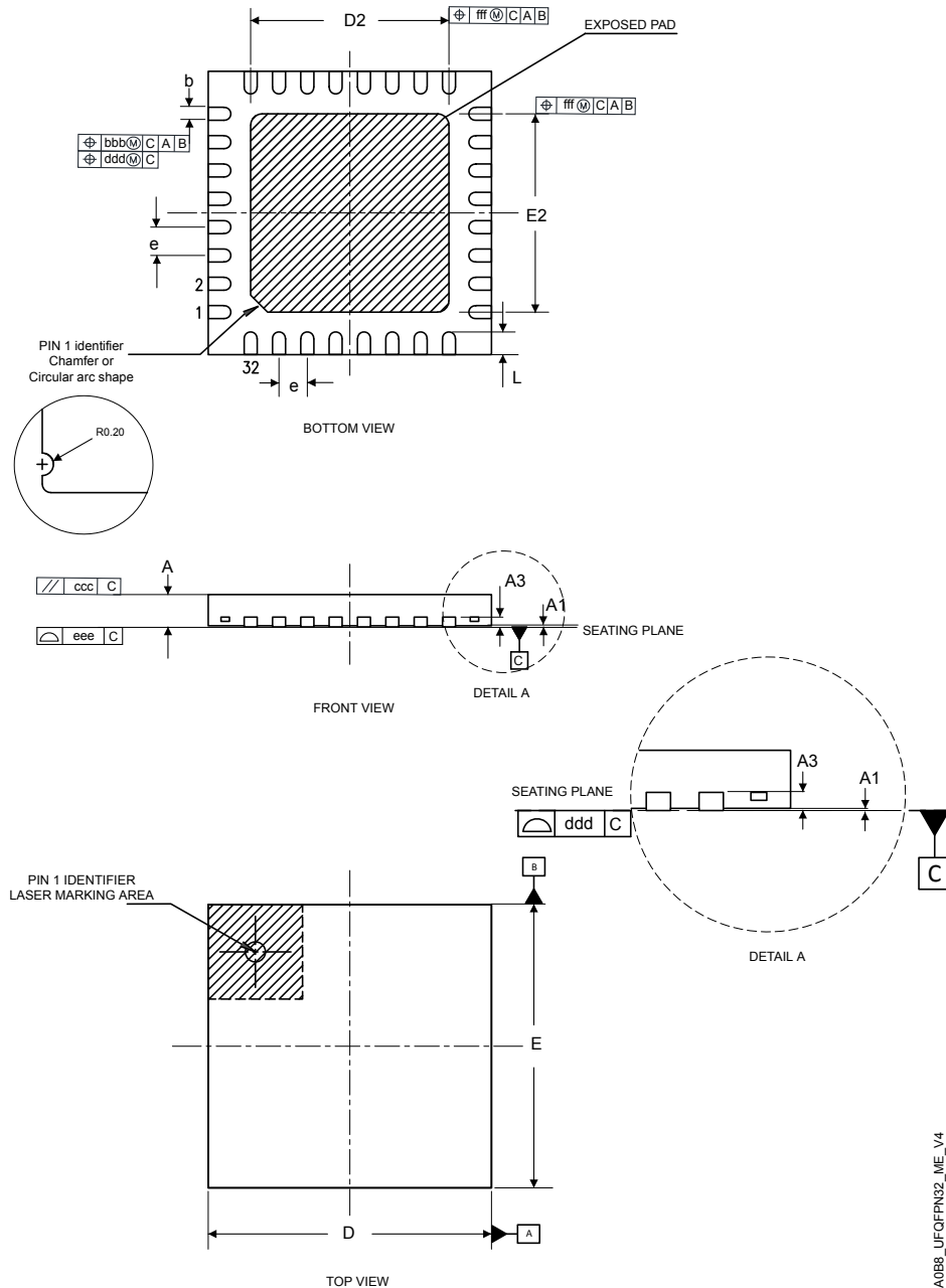
Figure 39. UFQFPN32 - Outline
