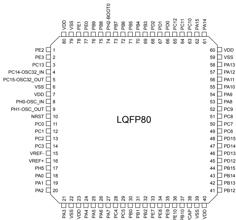
Figure 9. LQFP80 pinout
