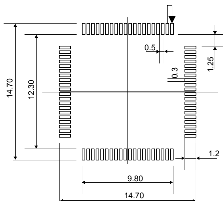
Figure 47. LQFP80 - Footprint example
