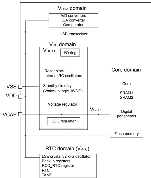
Figure 2. STM32C55xxx power supply overview
