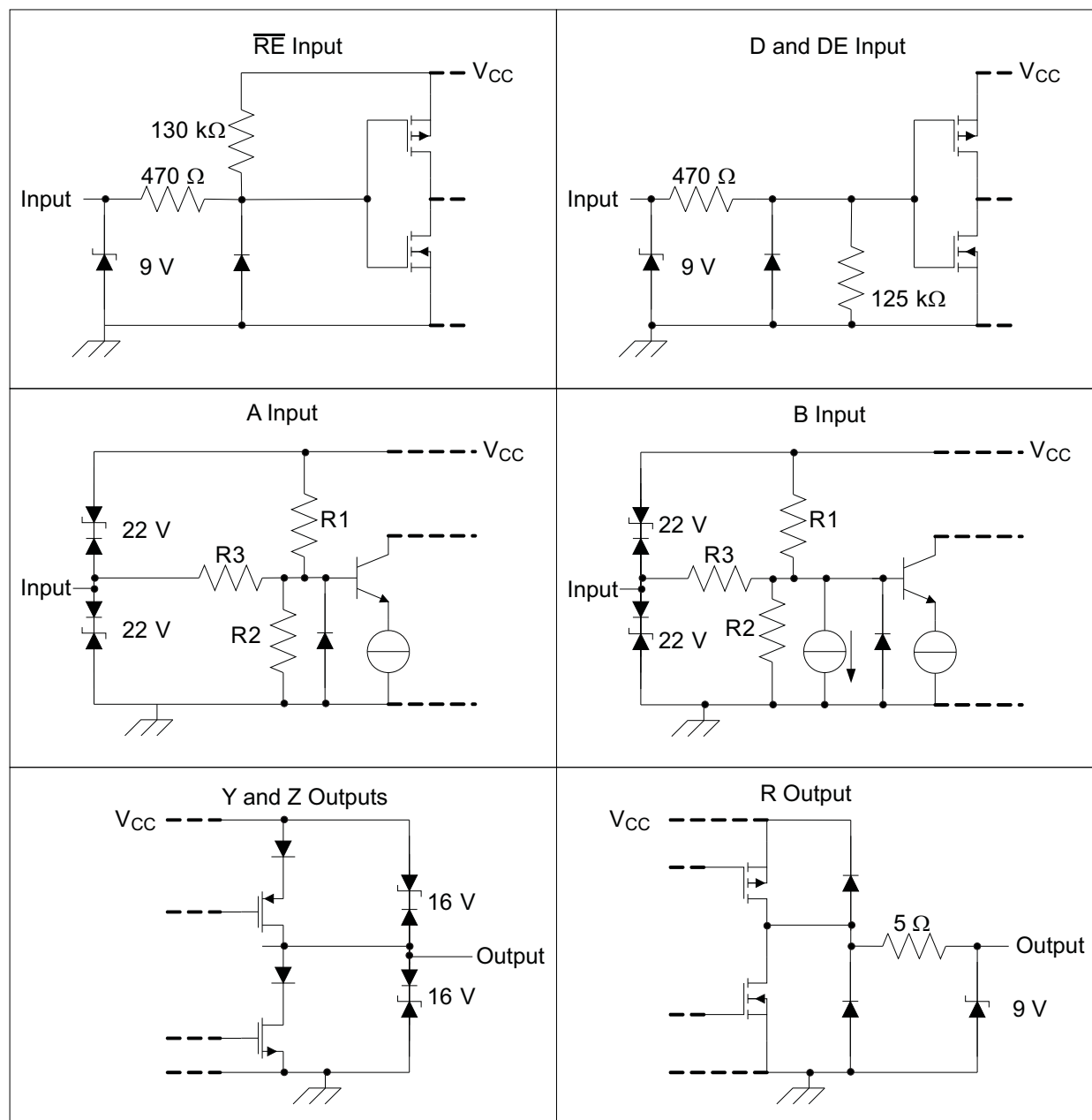
Figure 26. Equivalent Input and Output Schematic Diagrams
