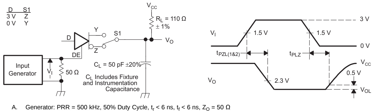
Figure 16. Driver Low-Level Output Enable and Disable Time Test Circuit and Voltage Waveforms
