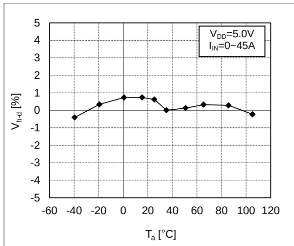
Figure 6. Temperature drift of sensitivity of CQ-206B (for reference, n=1 )
