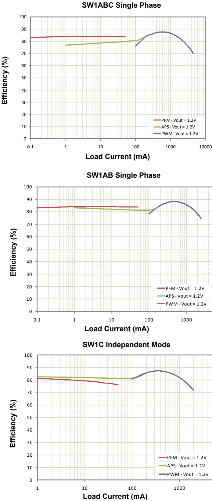
Figure 14. SW1AB and SW1C Efficiency Waveforms
