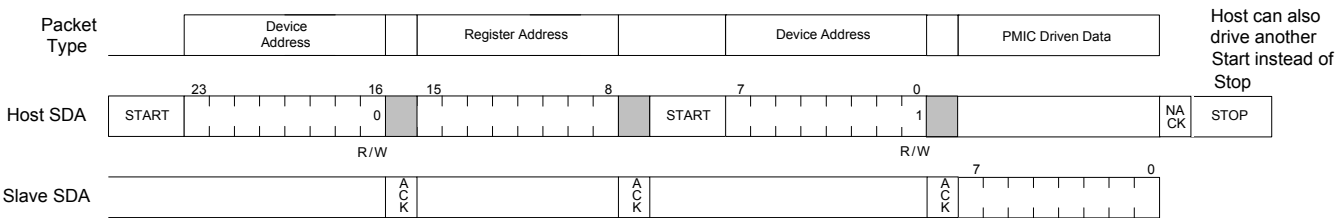
Figure 28. I 2 C Read Example
