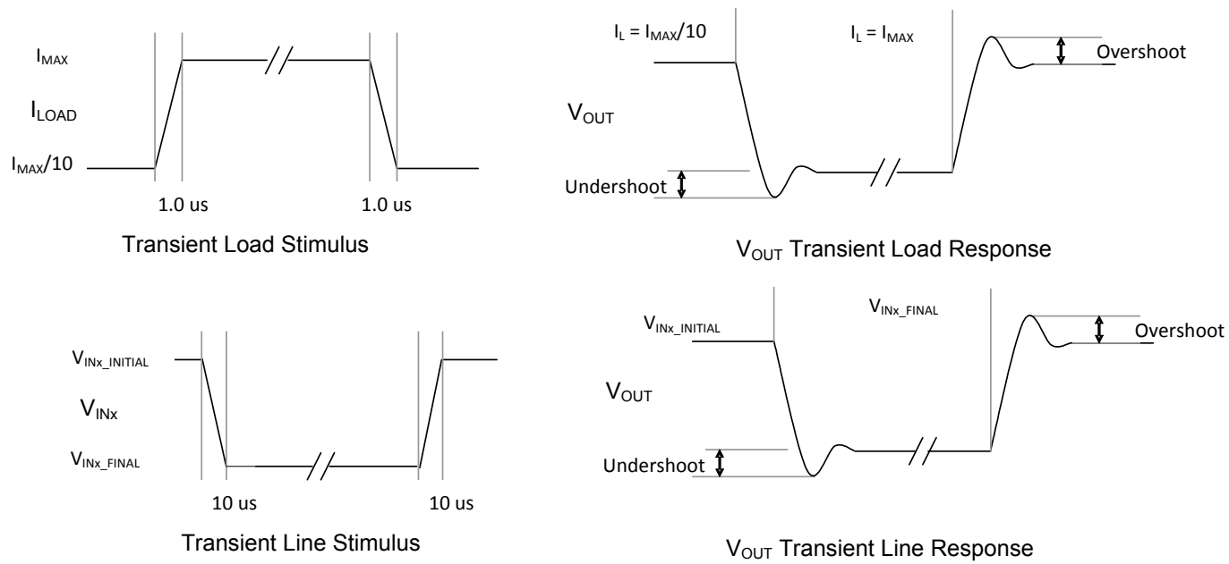
Figure 25. Transient Waveforms
