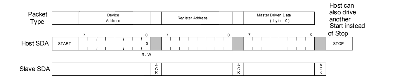
Figure 27. I 2 C Write Example
