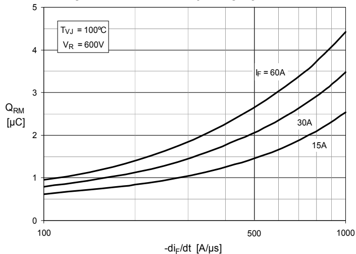
Fig. 23. Reverse Recovery Charge Q_{RM} vs. -di_F/dt
