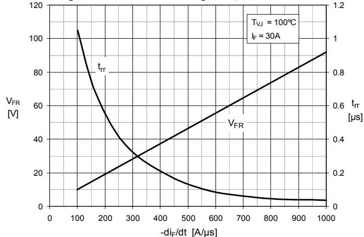
Fig. 27. Peak Forward Voltage V_{FR} , t_{rr} vs -di_F/dt
