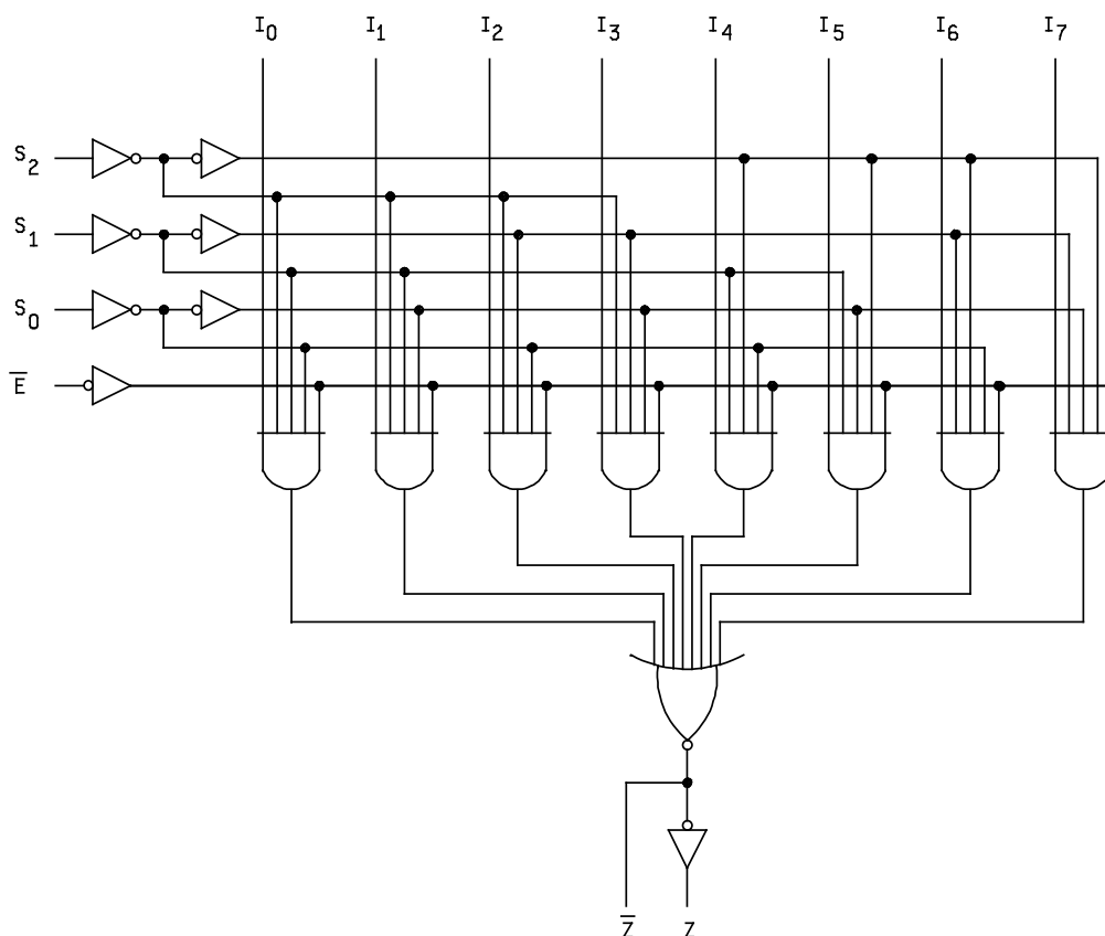
FIGURE 3. Logic diagram.
