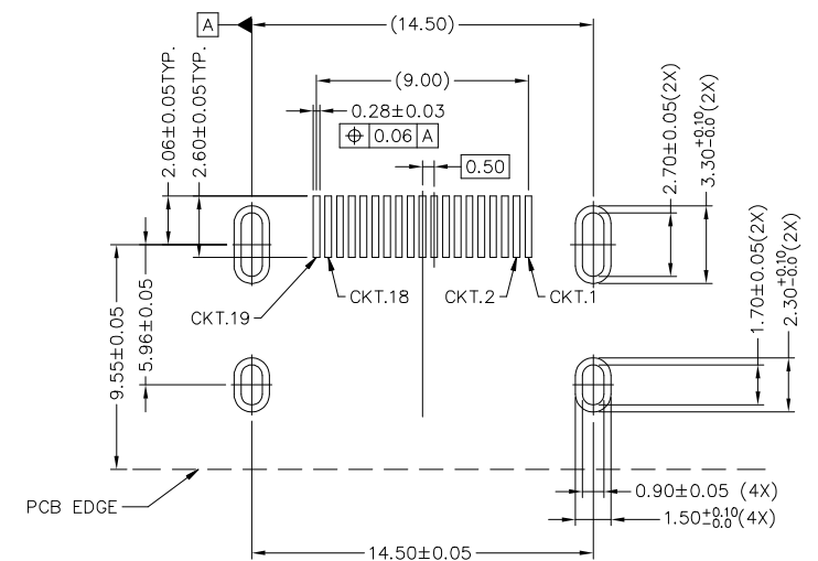
RECOMMENDED PCB LAYOUT CONNECTOR SIDE(TOP VIEW)
