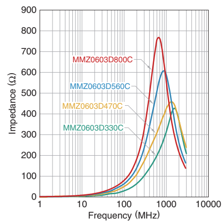
MMZ0603D series
