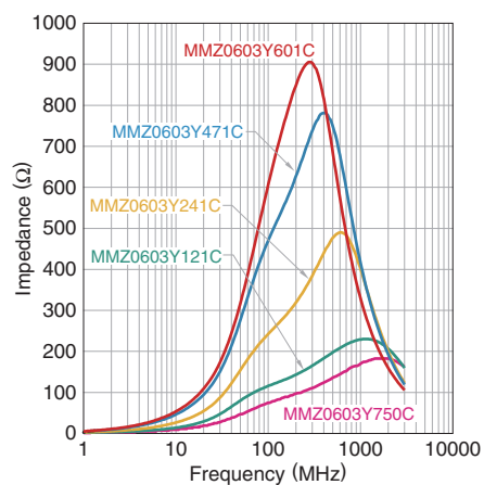
MMZ0603Y series
