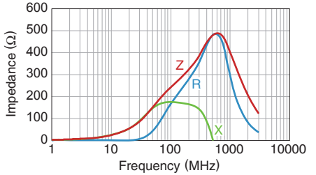
MMZ0603D330CTD25
