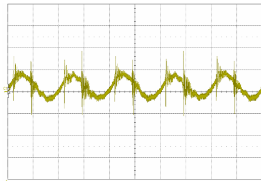
Figure 9. Output voltage ripple (20 mV/div.) at full rated load current into a resistive load with C_o = 10\text{ }\mu\text{F} tantalum + 1\text{ }\mu\text{F} ceramic and V_{in} = 48\text{V} . Time scale: 1µs/div.
