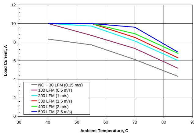
Figure 1. Available load current vs. ambient air temperature and airflow rates for SQE48T10120 converter mounted vertically with air flowing from pin 3 to pin 1, MOSFET temperature \leq 120^{\circ}\text{C} , V_{in} = 48\text{ V} .
