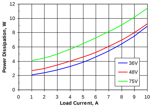
Figure 4. Power dissipation vs. load current and input voltage for SQE48T10120 converter mounted horizontally with air flowing from pin 1 to pin 8 at a rate of 300 LFM (1.5 m/s) and T_a = 25^\circ\text{C} .
