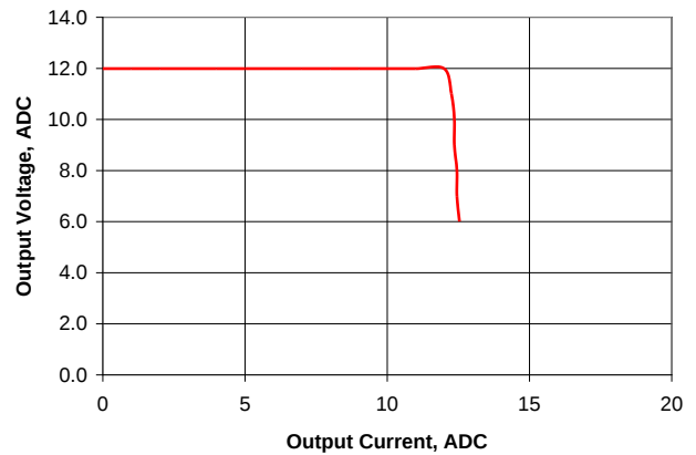
Figure 13. Output voltage vs. load current showing current limit point and converter shutdown point. Input voltage has almost no effect on current limit characteristic.
