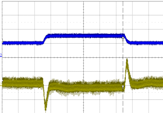
Figure 8. Output voltage response to load current step-change (5A - 7.5A - 5A) at V_{in} = 48\text{V} . Bottom trace: output voltage (50mV/div.). Top trace: load current (5A/div.). Current slew rate: 0.1\text{ A}/\mu\text{s} . C_o = 1\text{ }\mu\text{F} ceramic. Time scale: 0.1ms/div.
