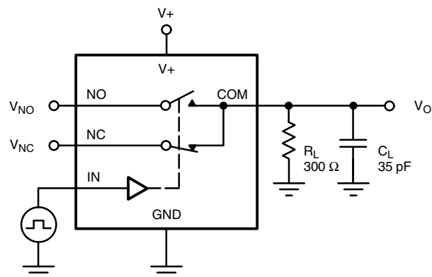
Fig. 2 - Break-Before-Make Interval
