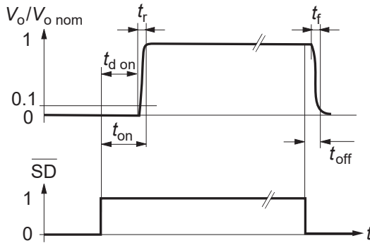
Fig. 5 Typical output response to the SD-signal.
