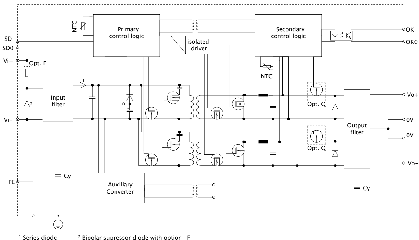
Fig. 1 Block diagram
