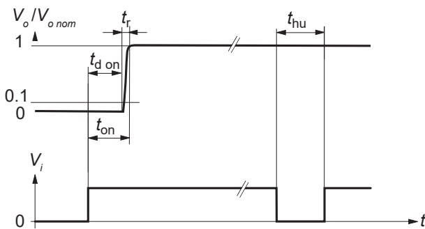
Fig. 6 Typical output response to V_i If option M is not fitted, t_{hu} = 0 ms.
