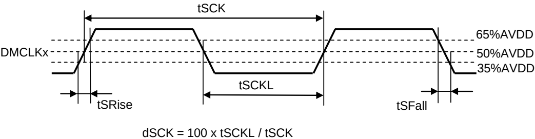
Figure 6. DMCLK1/2 Output Timing
