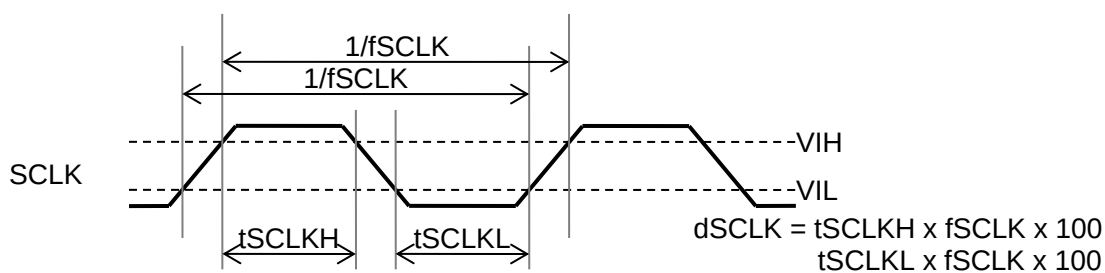
Figure 9. SPI Interface SCLK
