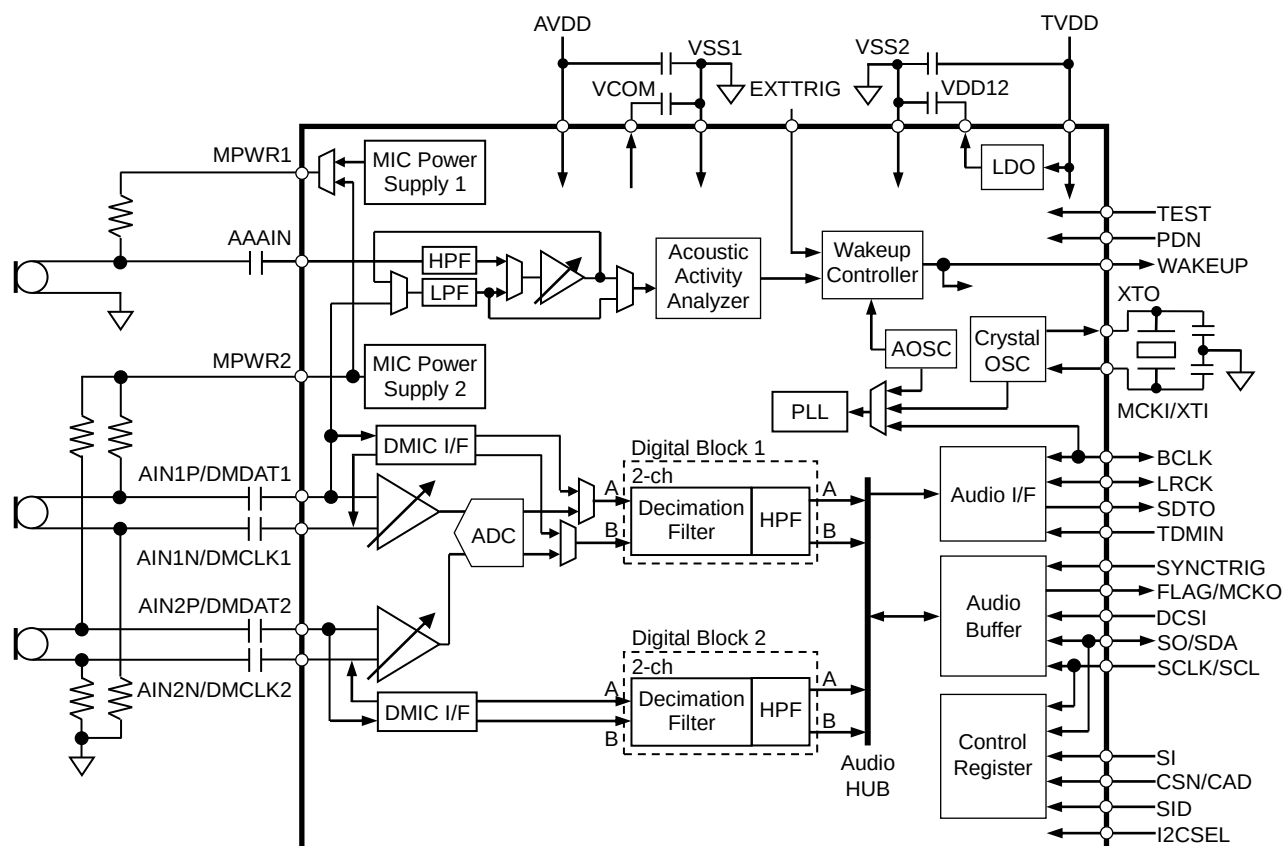
Figure 1. AK5706 Block Diagram
