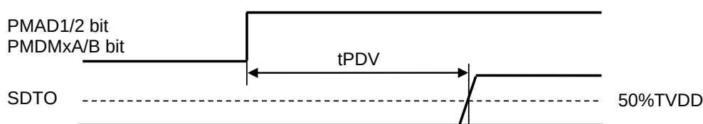
Figure 15. ADC, DMIC1/2 Power Up Timing
