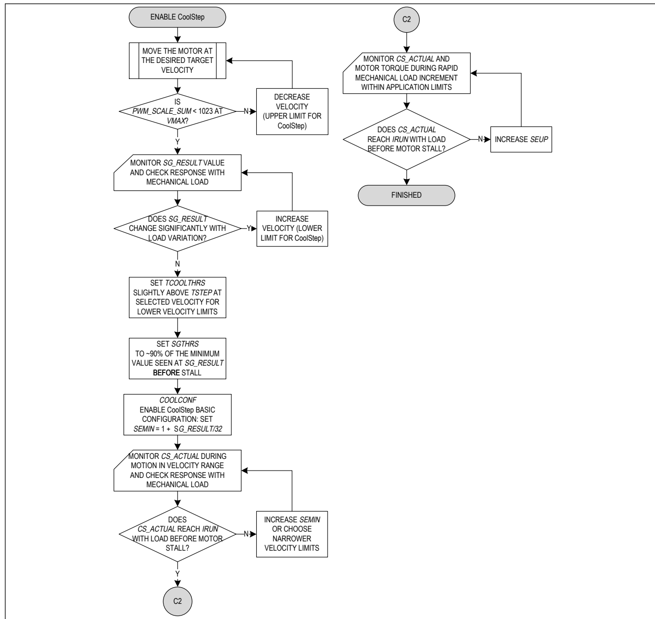
Figure 42. Quick Configuration Guide for CoolStep with StealthChop2
