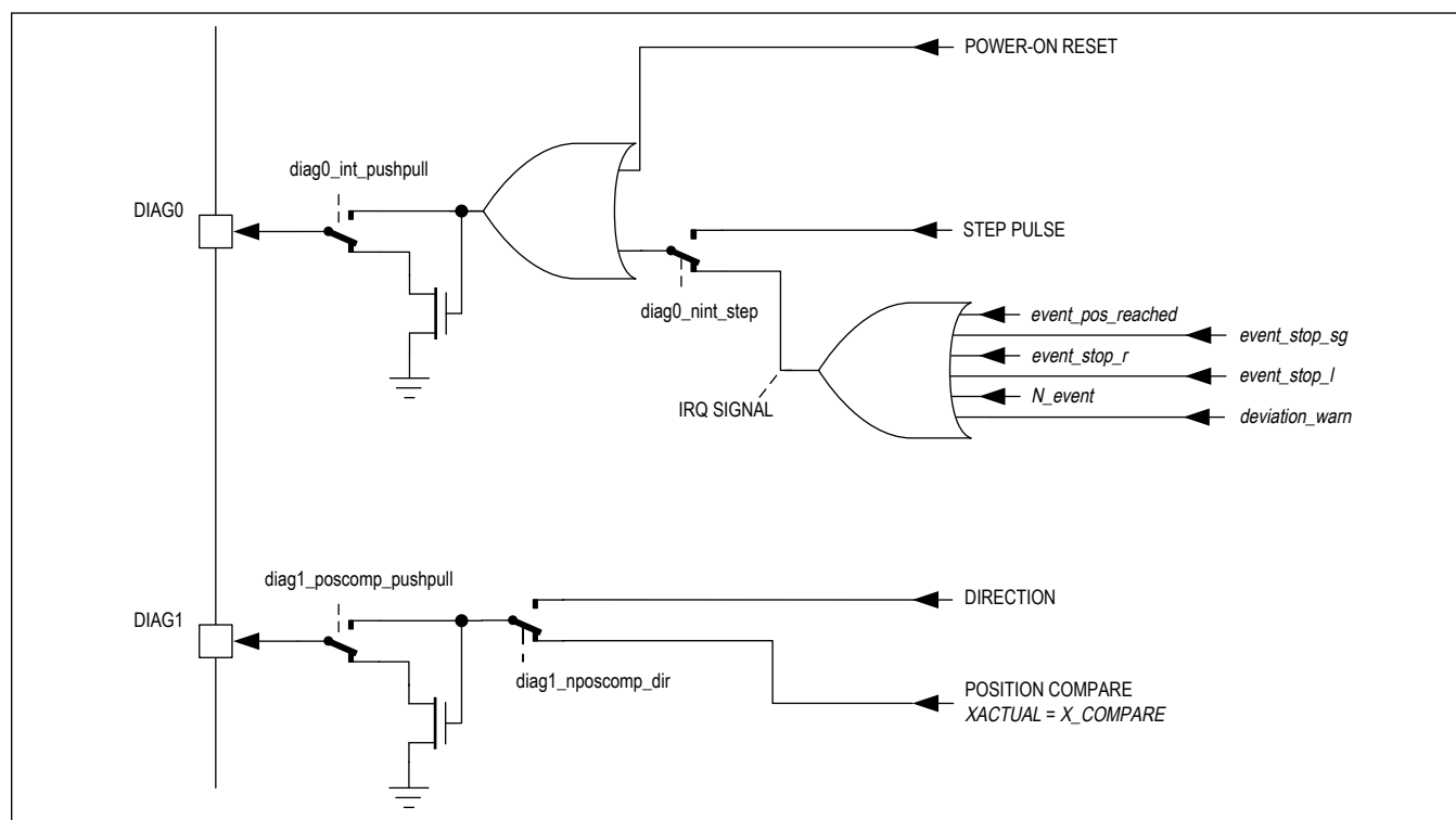
Figure 32. Diagnostic Outputs Configuration Options
