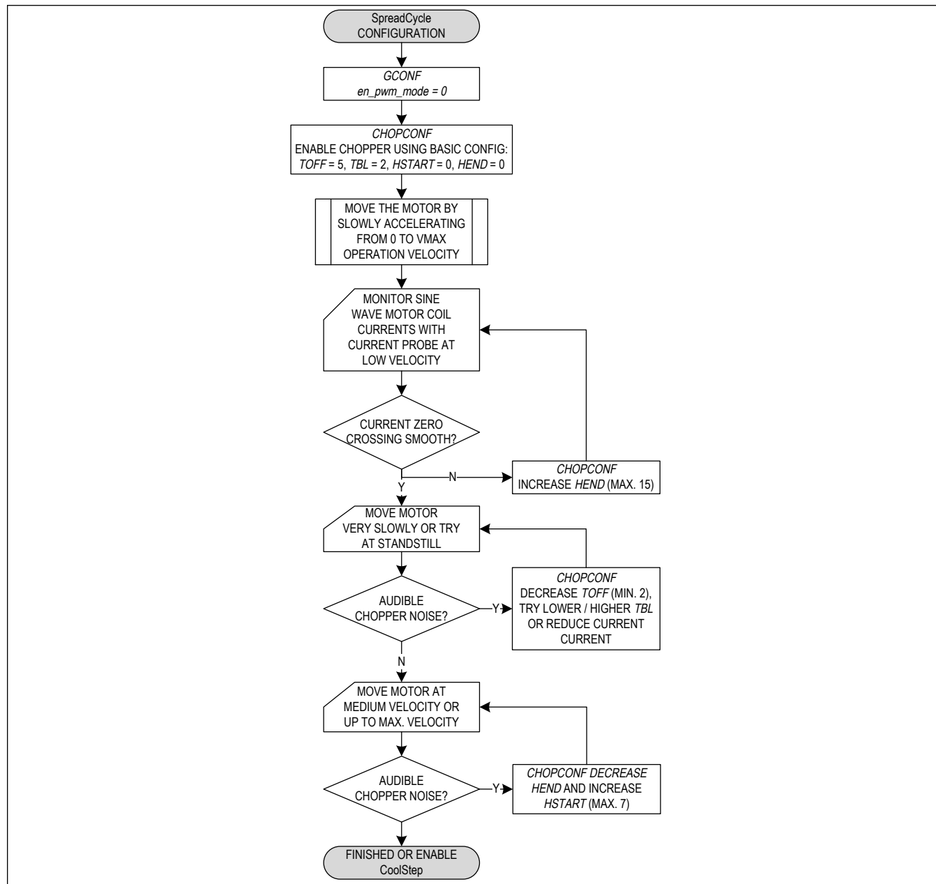
Figure 41. Quick Configuration Guide for SpreadCycle
