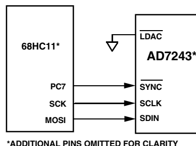
Figure 15. AD7243–68HC11 Interface
