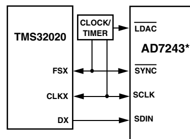
Figure 13. AD7243–TMS32020 Interface
