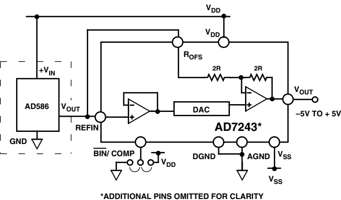
Figure 10. Bipolar Configuration with External Reference
