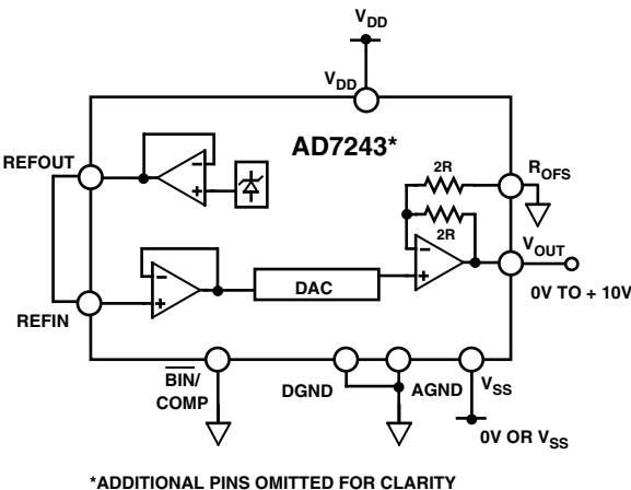
Figure 9. Unipolar (0 V to +10 V) Configuration
