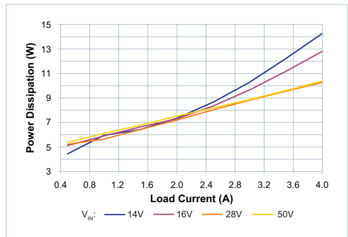
Figure 10 — Power dissipation at 25^{\circ}\text{C} case temperature, V_{OUT} = 50\text{V}
