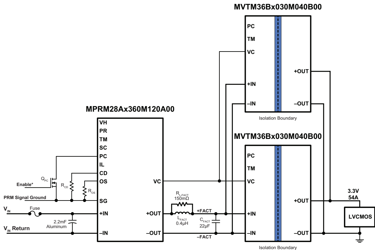
MPRM28Ax360M120A00 + two MVTM36Bx030M040B00s for isolated 180W-logic supply
