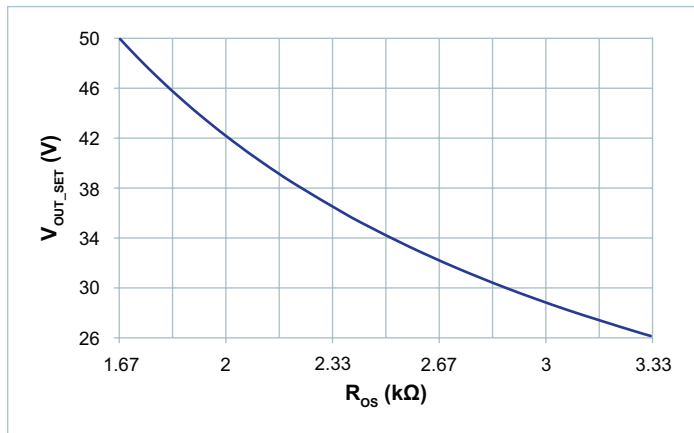
Figure 23 — PRM output voltage set point determined by value of R_{OS}
