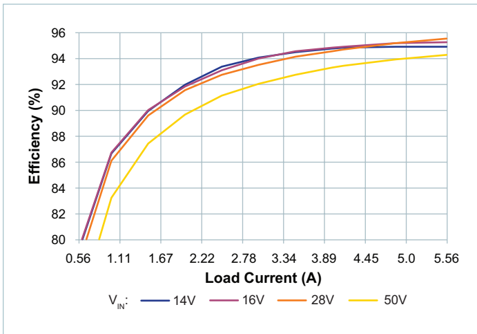
Figure 5 — Efficiency at 25^{\circ}\text{C} case temperature, V_{OUT} = 26\text{V}
