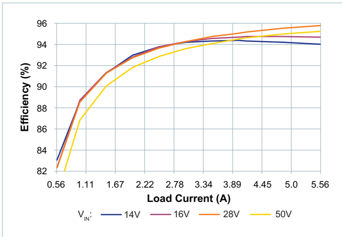
Figure 7 — Efficiency at 25^{\circ}\text{C} case temperature, V_{OUT} = 36\text{V}
