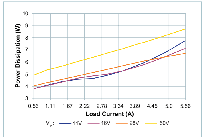
Figure 6 — Power dissipation at 25^{\circ}\text{C} case temperature, V_{OUT} = 26\text{V}
