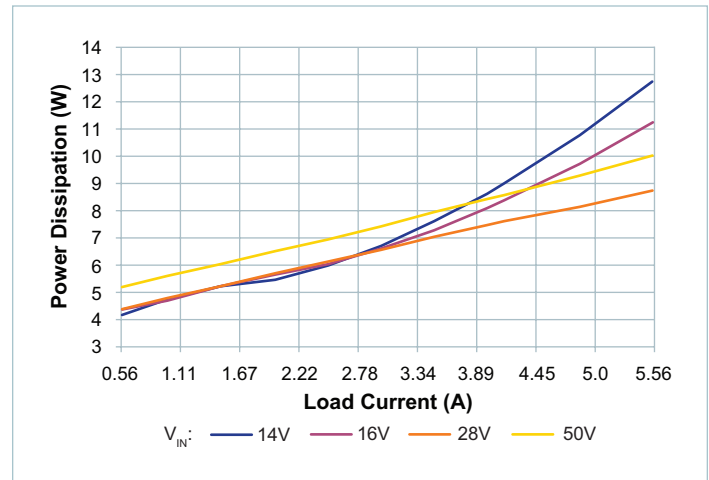
Figure 8 — Power dissipation at 25^{\circ}\text{C} case temperature, V_{OUT} = 36\text{V}
