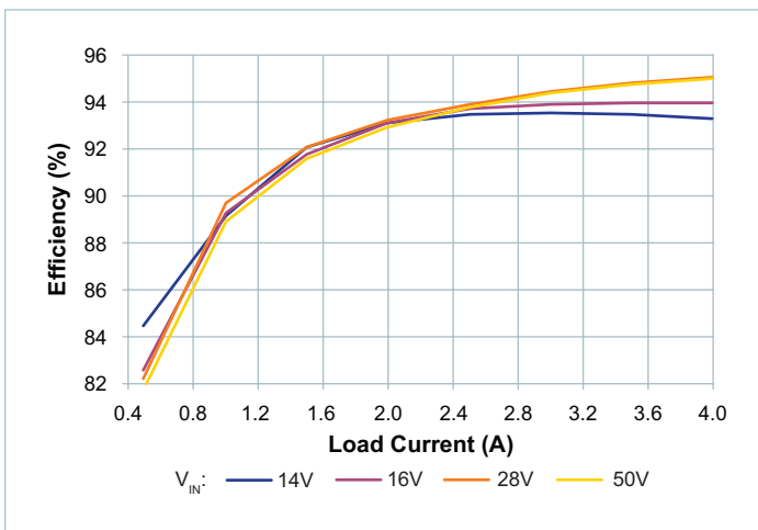
Figure 9 — Efficiency at 25^{\circ}\text{C} case temperature, V_{OUT} = 50\text{V}
