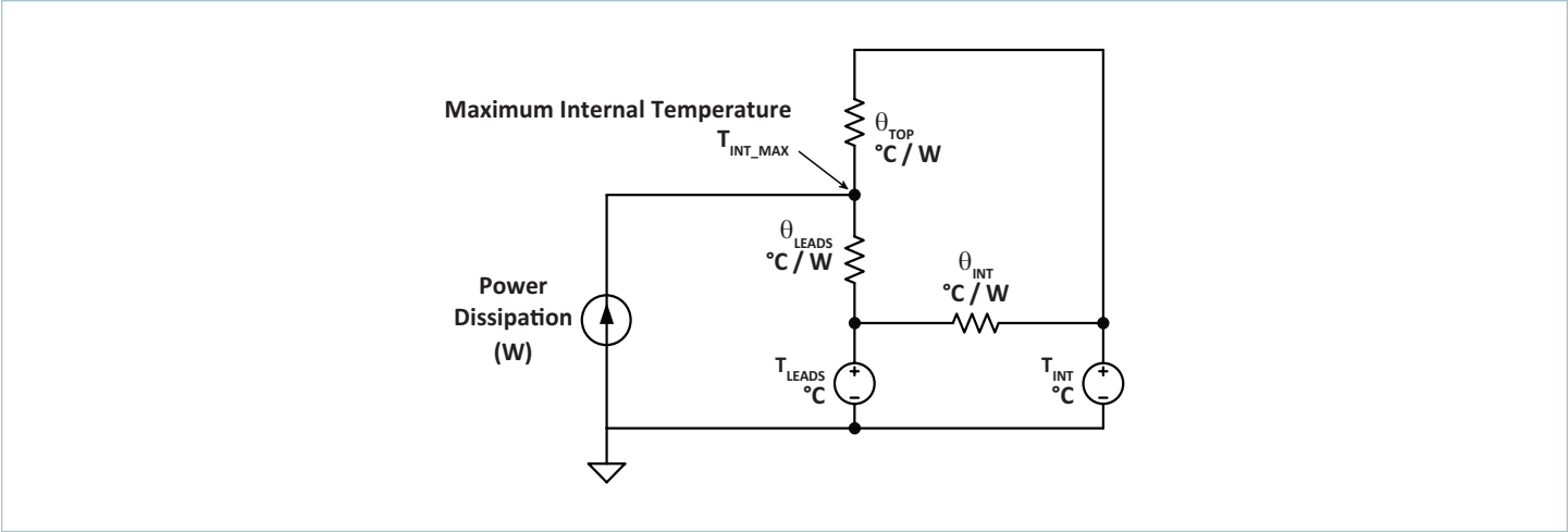
Figure 29 — Thermal model
