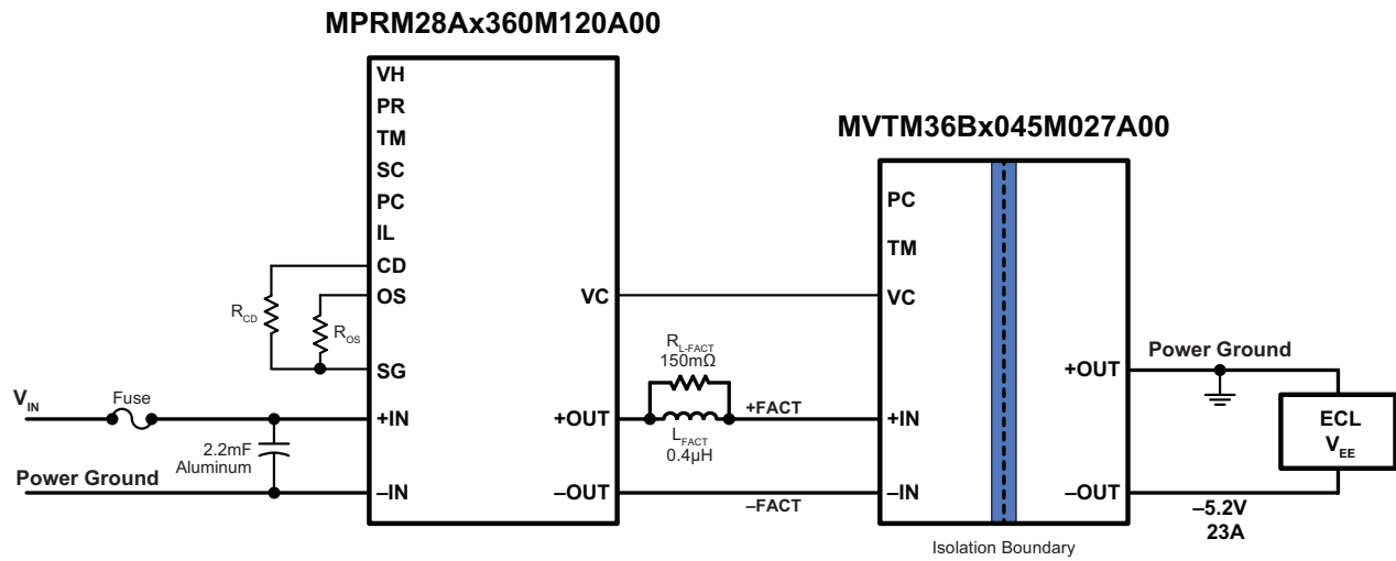
MPRM28Ax360M120A00 + MVTM36Bx045M027A00 isolated adaptive-loop configuration for negative supply
