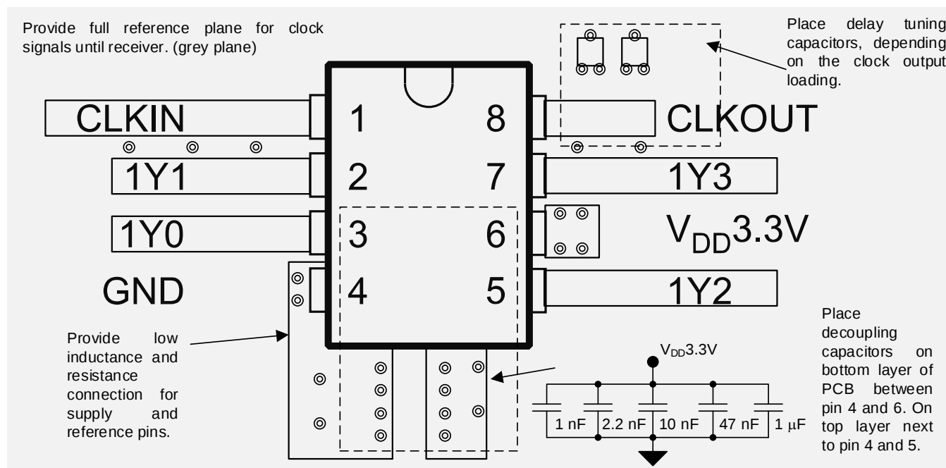
Figure 12. Layout Illustration
