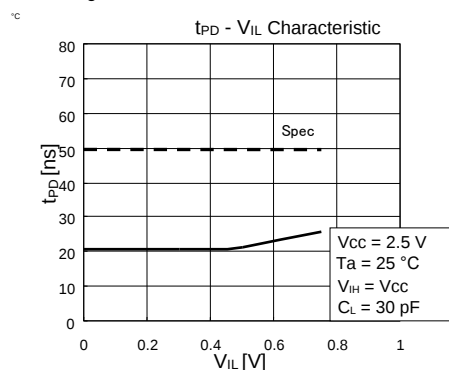
Figure 60. V_{IL} dependency of Data Output Delay Time t_{PD}
