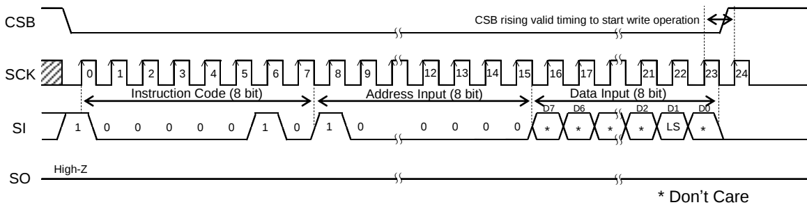
Figure 51. Lock ID Page Command
