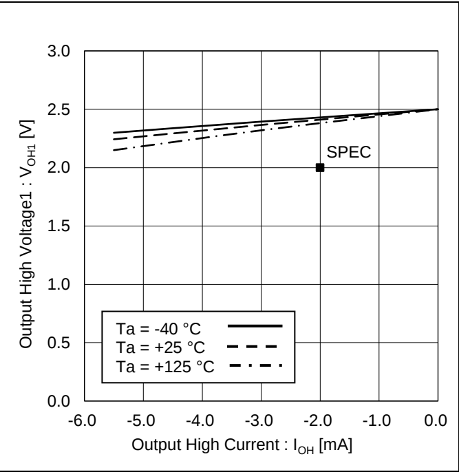
Figure 11. Output High Voltage1 vs Output High Current ( V_{CC} = 2.5 V)
