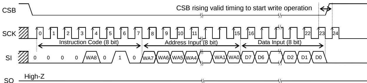
Figure 43. Write Command (Byte Write)
