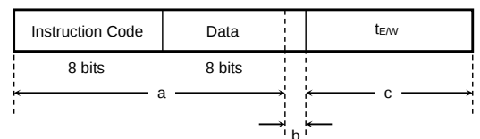
Figure 56. WRSR Cancel Valid Timing
