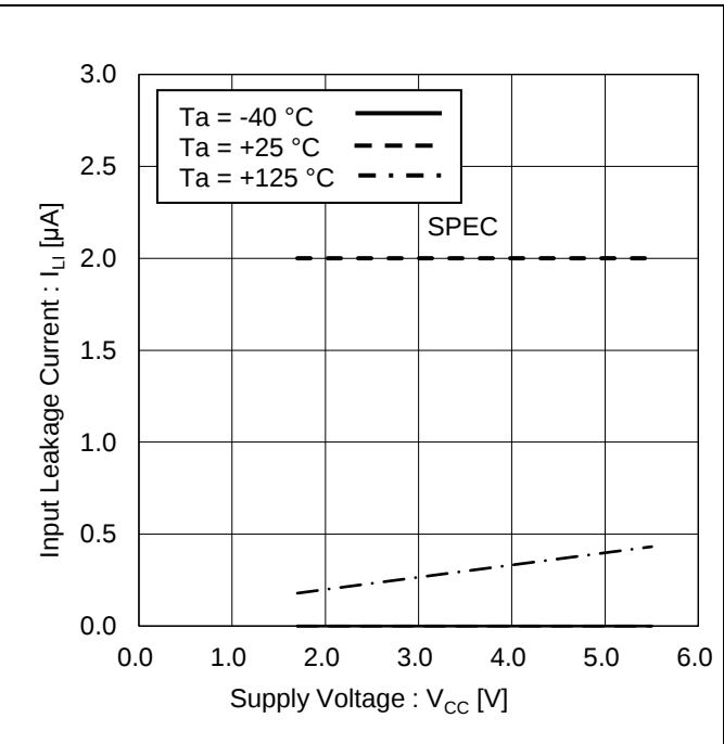
Figure 13. Input Leakage Current vs Supply Voltage (CSB, SCK, SI, HOLDB, WPB)
