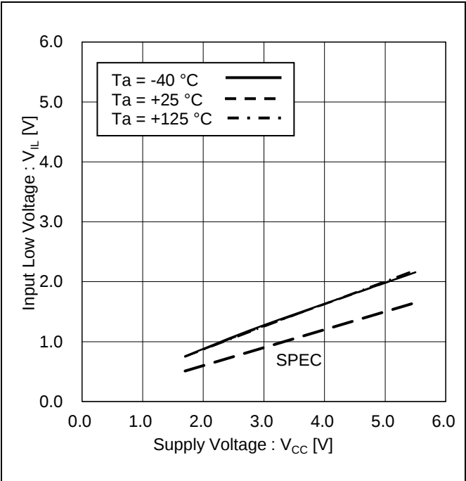
Figure 8. Input Low Voltage vs Supply Voltage (CSB, SCK, SI, HOLDB, WPB)
