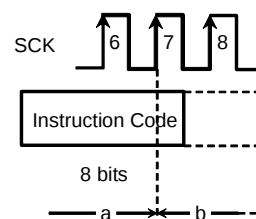
Figure 57. WREN/WRDI Cancel Valid Timing
