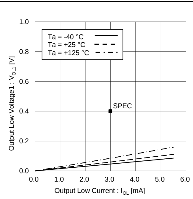
Figure 9. Output Low Voltage1 vs Output Low Current ( V_{CC} = 2.5\text{ V} )
