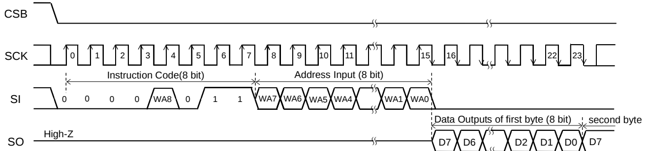
Figure 42. Read Command
