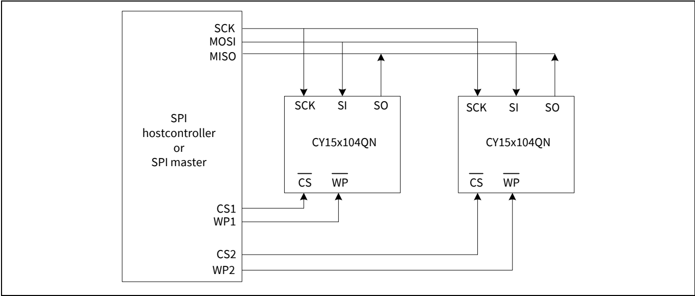
Figure 3 System configuration with SPI port
