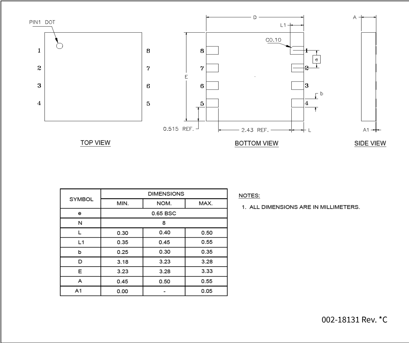
Figure 27 8-pin GQFN (3.23 × 3.28 × 0.55 mm) LP08A package outline, 002-18131
