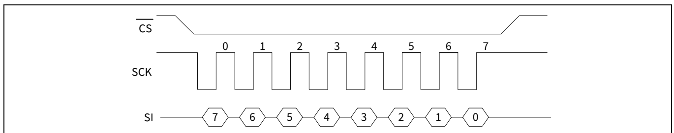
Figure 6 SPI mode 3
