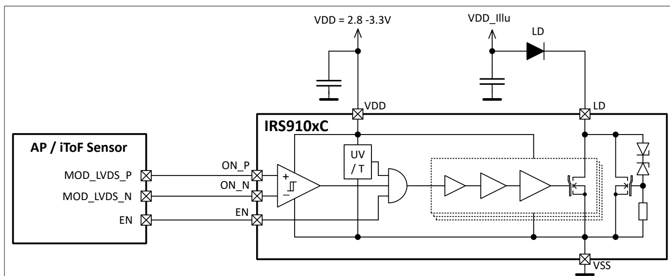
Figure 2 IRS9100C Application Circuitry
