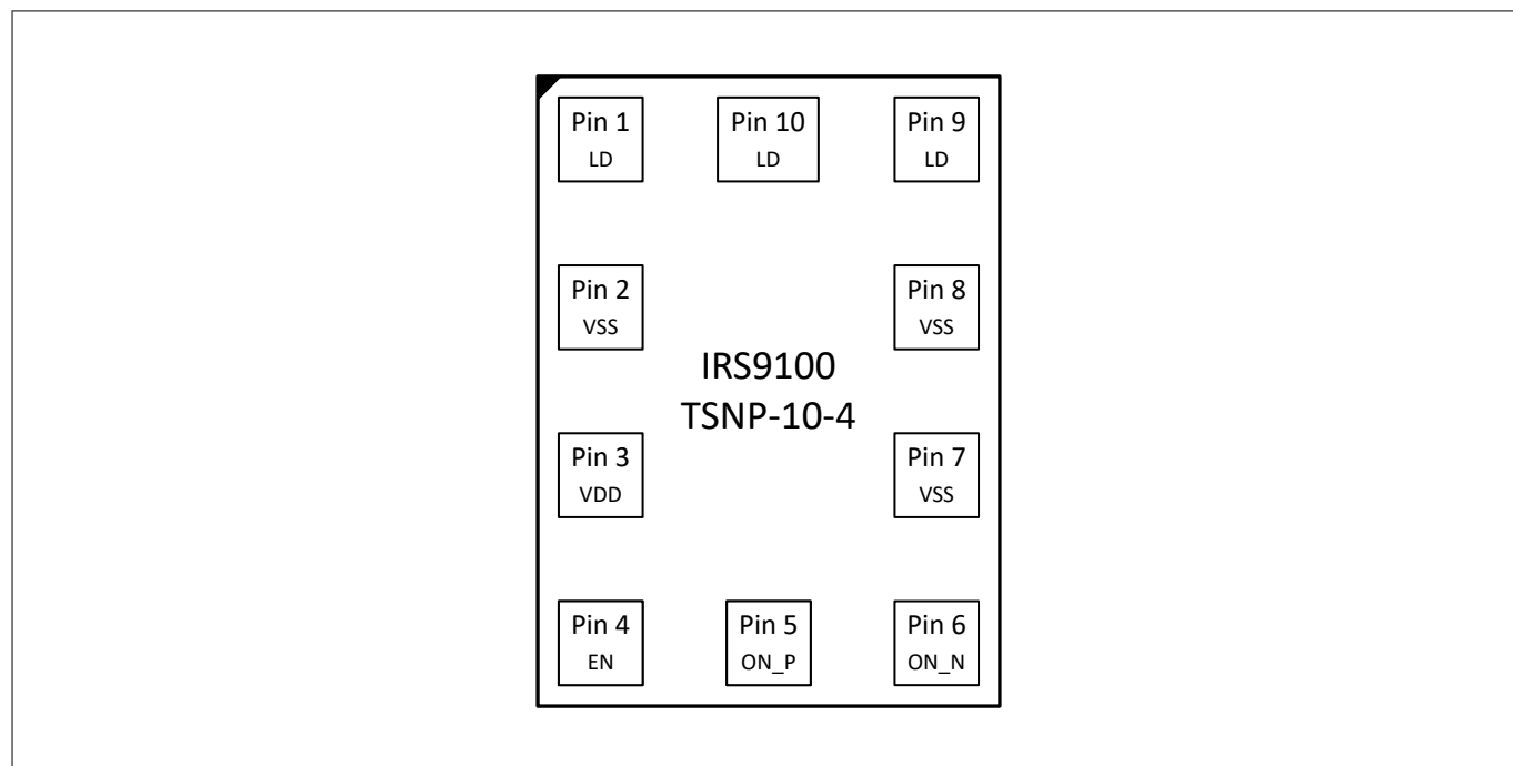
Figure 3 Pin-out
