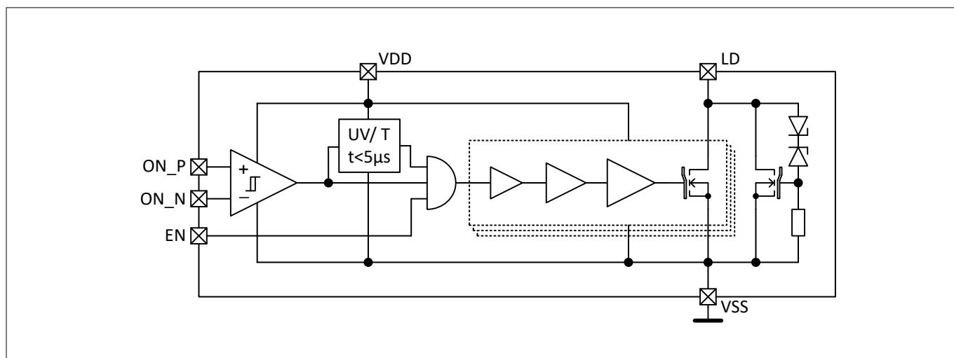
Figure 1 IRS9100C Block diagram
