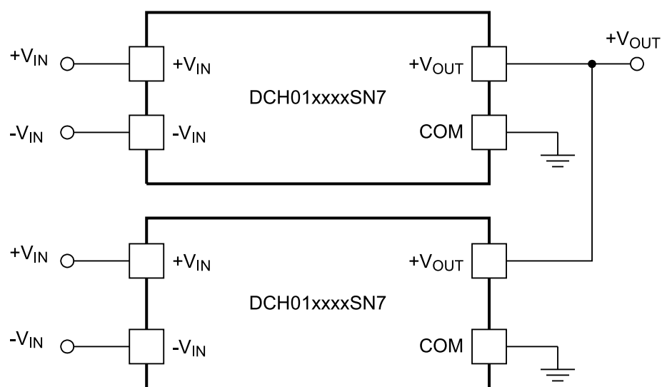
Figure 26. Connecting Multiple DCH01s in Parallel
