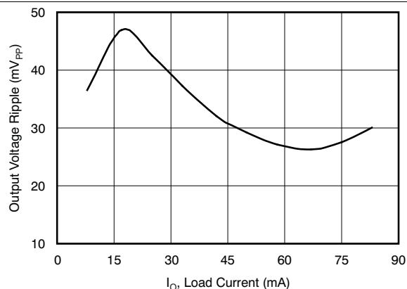
Figure 11. DCH010512S Ripple Voltage
