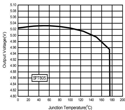
Figure 5. Output Voltage vs. Junction Temperature
