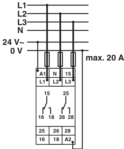
Connection diagram
