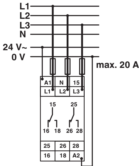
Application drawing
