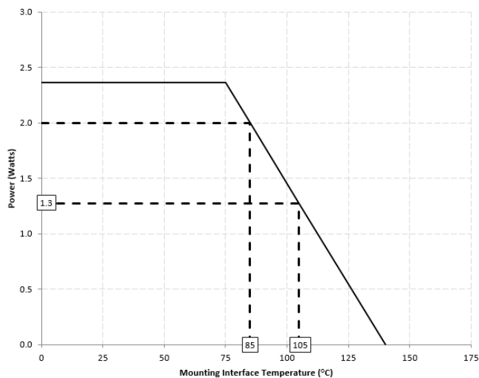
DC0710J5020AHF Power Derating Curve
