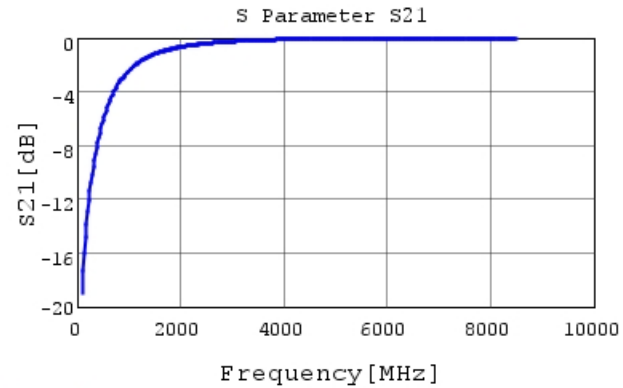
GCQ1555C1H1R8WB01 S21 DCOV, 25degC
