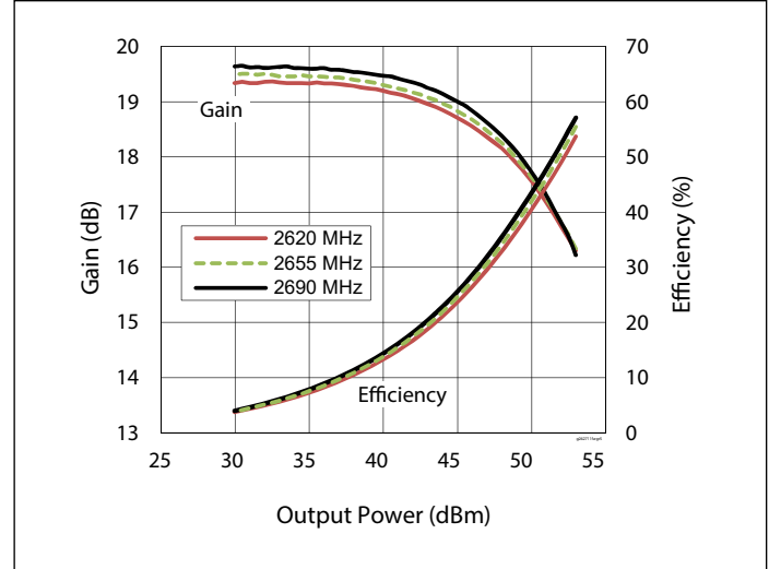
Figure 8. CW Performance
