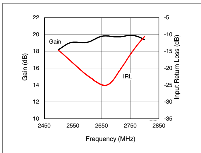
Figure 10. CW Performance Small Signal Gain & Input Return Loss
