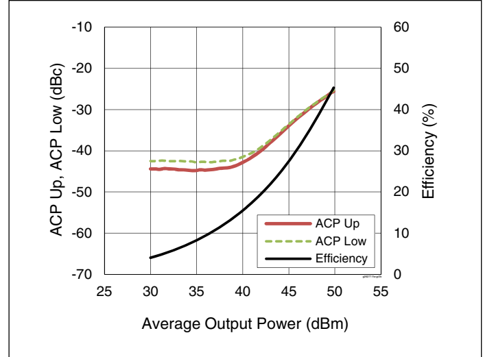
Figure 4. Single-carrier WCDMA Drive-up
