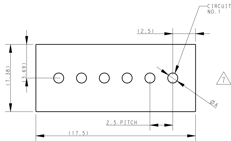
PCB MOUTING LAYOUT
