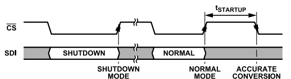
Figure 69. Shutdown Mode Operation
