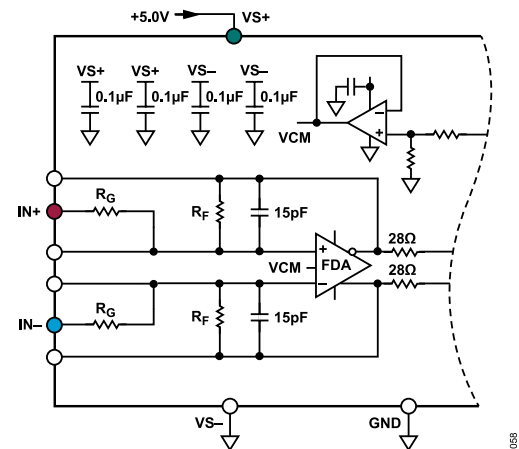
Figure 58. ADAQ4381-4 Configured at Fully Differential Inputs
