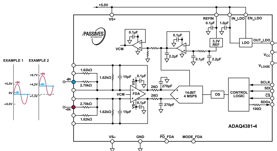
Figure 53. Single-Ended Input Configuration with Gain = 0.6, \pm 5.5\text{ V} Input, V_S = 5\text{ V}
