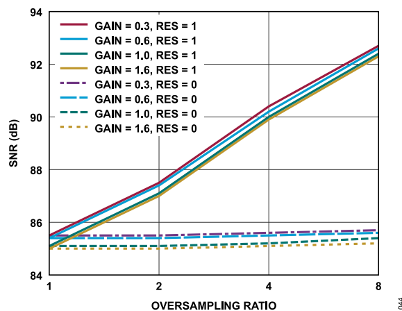
Figure 44. SNR vs. Rolling Average Oversampling, f_{IN} = 1 kHz
