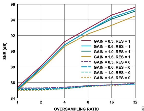
Figure 41. SNR vs. Normal Average Oversampling, f_{IN} = 1 kHz
