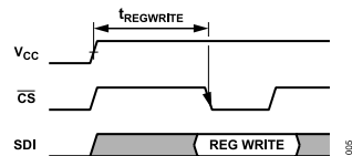
Figure 5. Power-Up Time to Register Read Write Access
