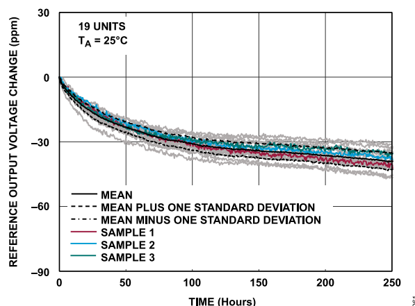
Figure 62. ADAQ4381-4 Internal Reference Early Life Drift
