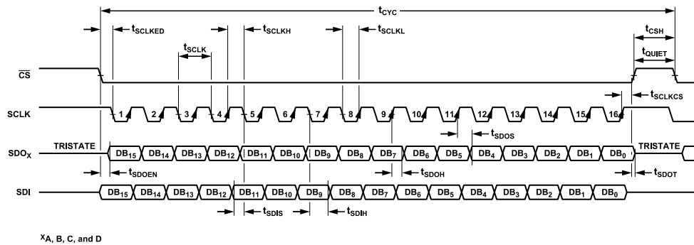
Figure 2. Serial Interface Timing Diagram
