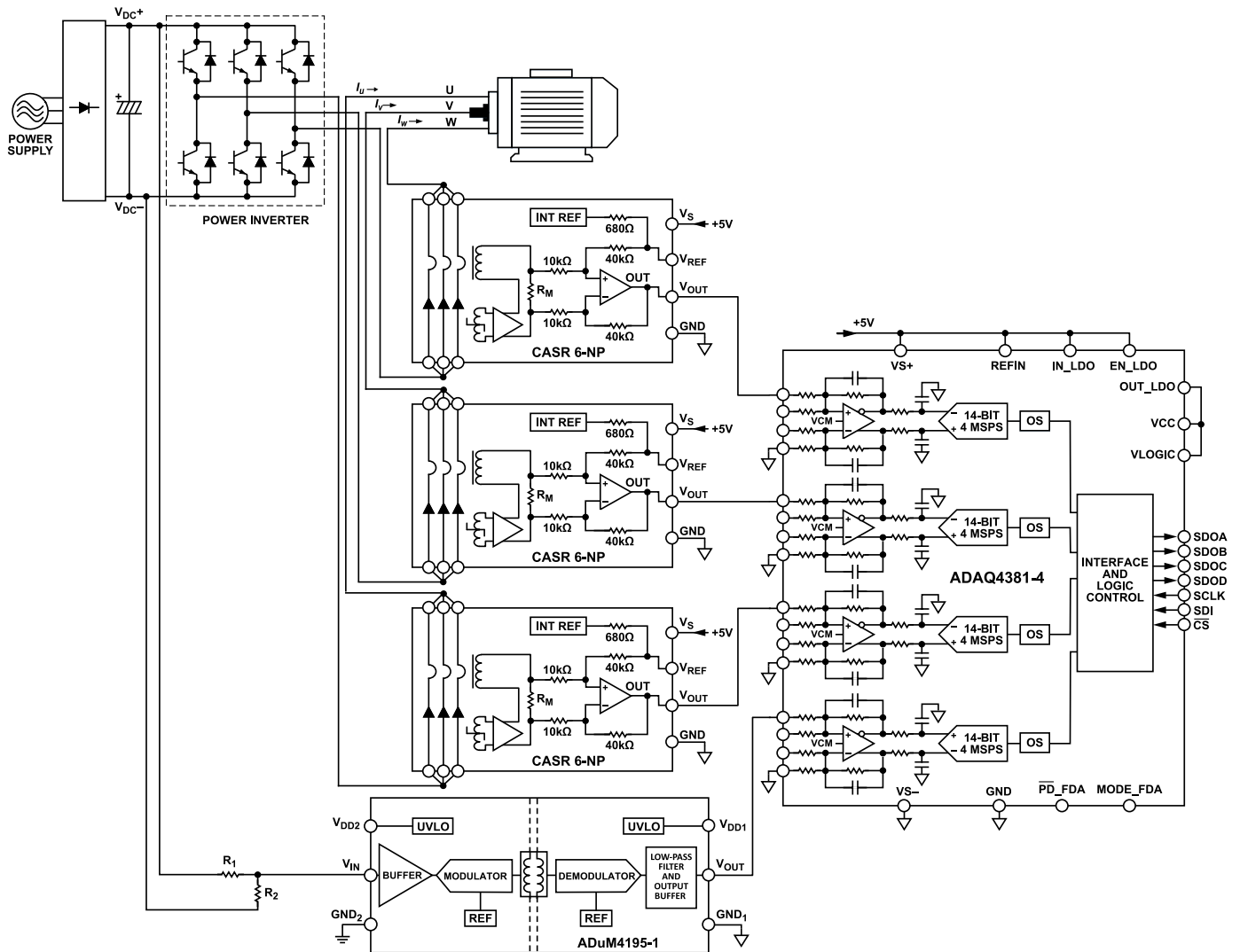
Figure 1. Precision Current and Voltage Sensing for Servo Motors Control Using ADAQ4381-4
