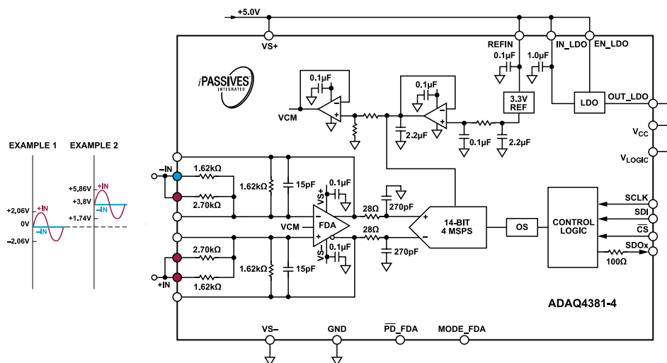
Figure 55. Single-Ended Input Configuration with Gain = 1.6, \pm 2.06 V Input, V_S = 5 V
