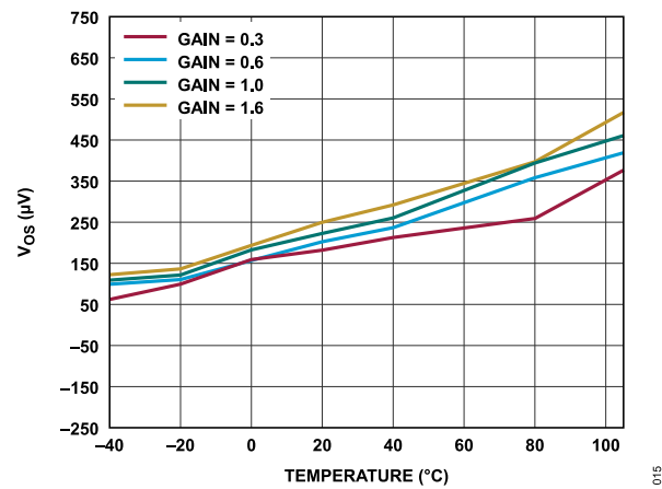
Figure 15. Offset Error vs. Temperature
