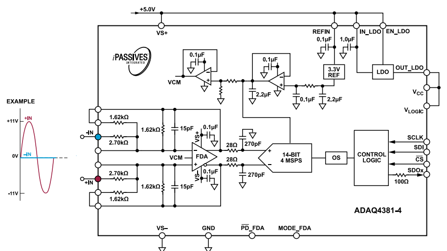
Figure 52. Single-Ended Input Configuration with Gain = 0.3, \pm 11\text{ V} Input, V_S = 5\text{ V}
