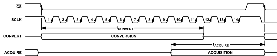
Figure 3. Internal Conversion Acquire Timing
