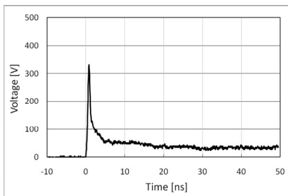
ESD Waveform (IEC61000-4-2:8kV Contact)
