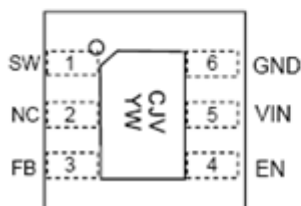
Top View U-DFN2020-6 (Type C)
