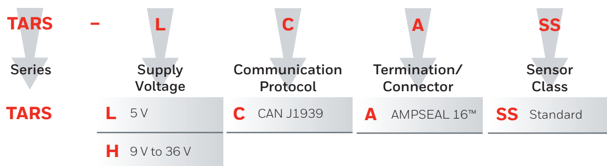
FIGURE 2. PRODUCT NOMENCLATURE
