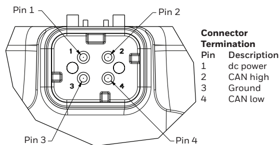
FIGURE 5. PINOUT
