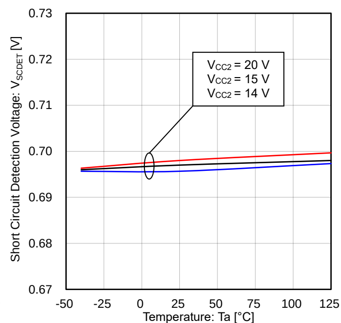
Figure 48. Short Circuit Detection Voltage vs Temperature
