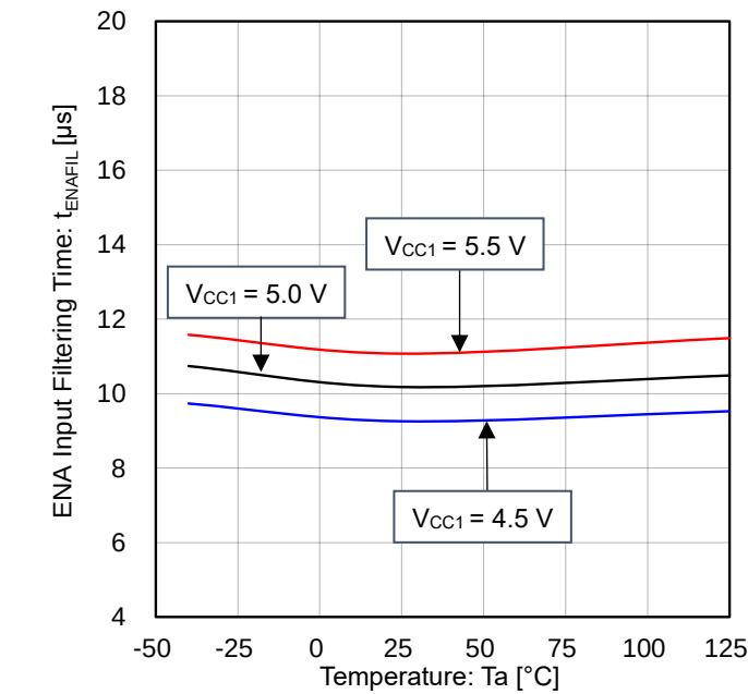
Figure 15. ENA Input Filtering Time vs Temperature
