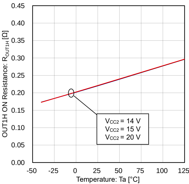
Figure 16. OUT1H ON Resistance vs Temperature
