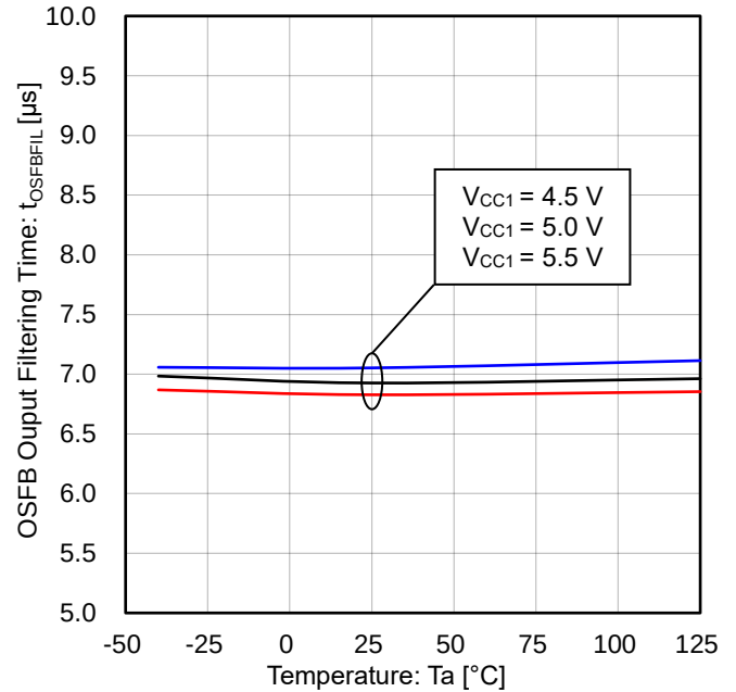
Figure 52. OSFB Output Filtering Time vs Temperature
