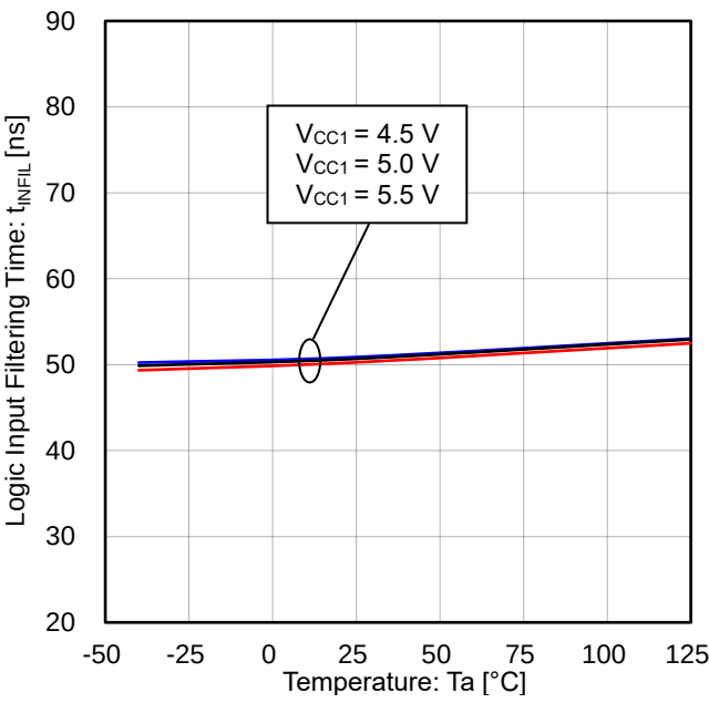
Figure 14. Logic Input Filtering Time vs Temperature
