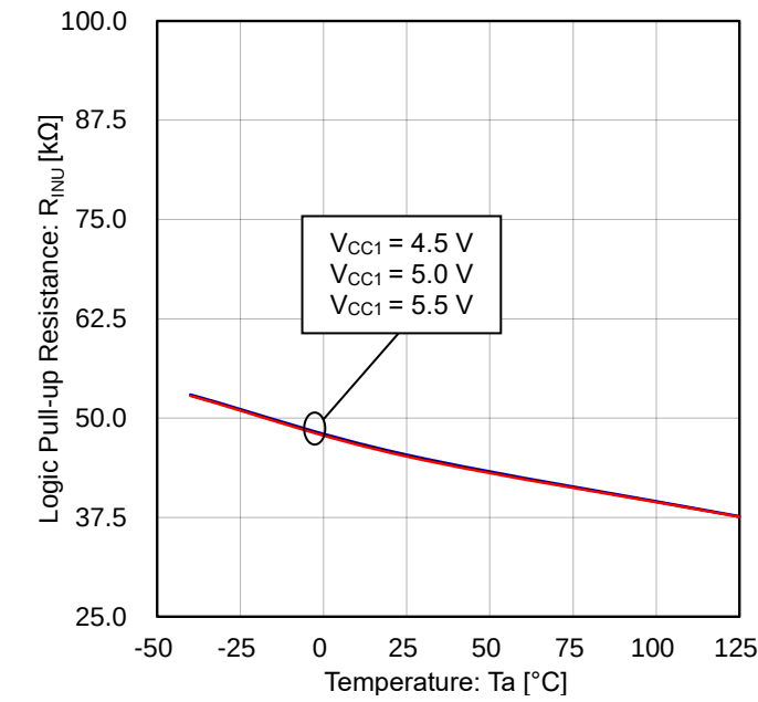
Figure 13. Logic Pull-up Resistance vs Temperature
