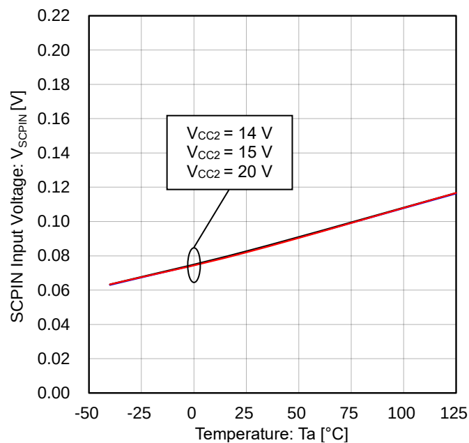
Figure 46. SCPIN Input Voltage vs Temperature
