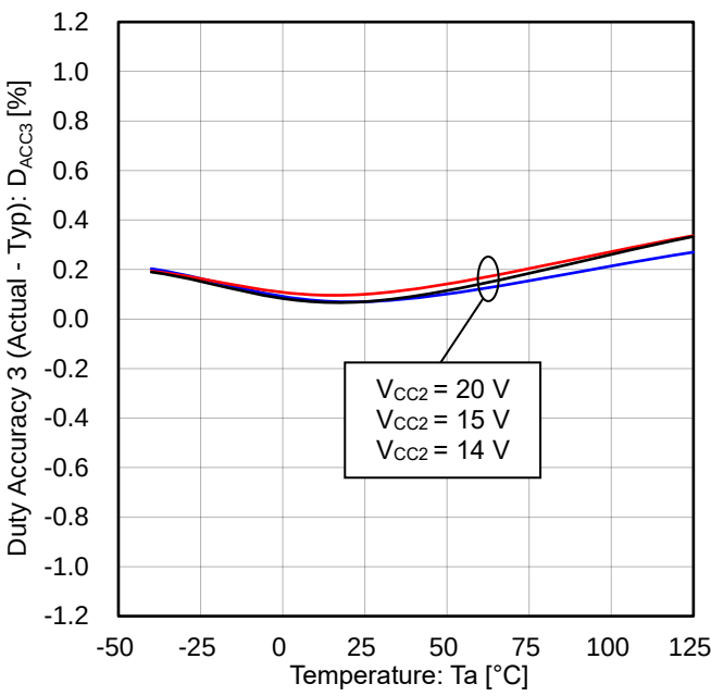
Figure 36. Duty Accuracy 3 (Actual - Typ) vs Temperature
