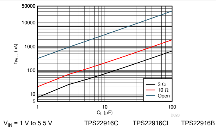
Figure 6-35. Fall Time
