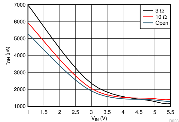
Figure 6-28. Slow Turn-On vs Load Resistance
