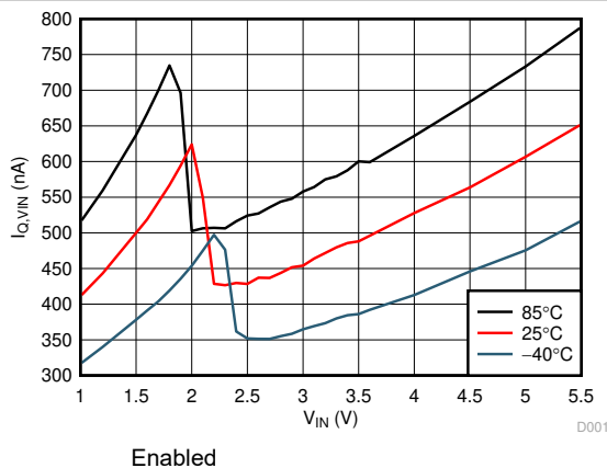
Figure 6-5. Quiescent Current
