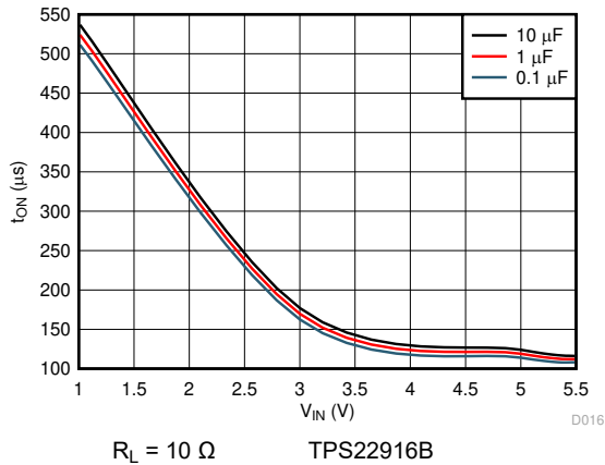
Figure 6-15. Fast Turn-On vs Load Capacitance
