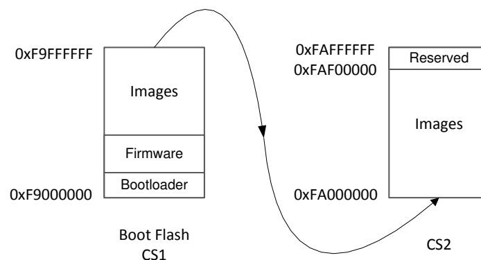
Figure 24. Two 16-Mbit Flash Memory Components
