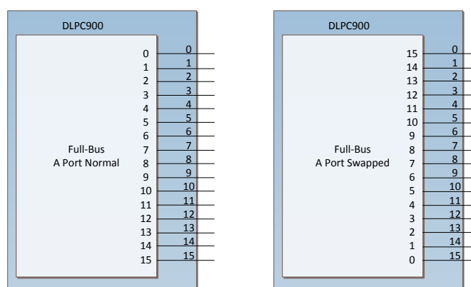
Figure 18. Controller to DMD Full-Bus Connections
