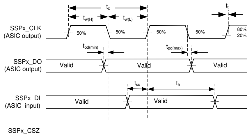
Figure 11. Synchronous Serial Port Interface – Slave (Modes 0/3)
