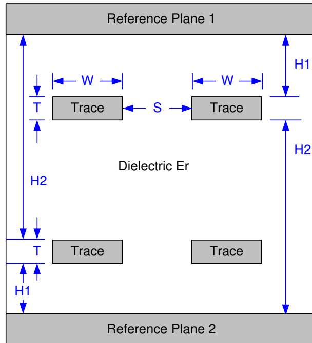
Figure 41. PCB Stackup Geometries
