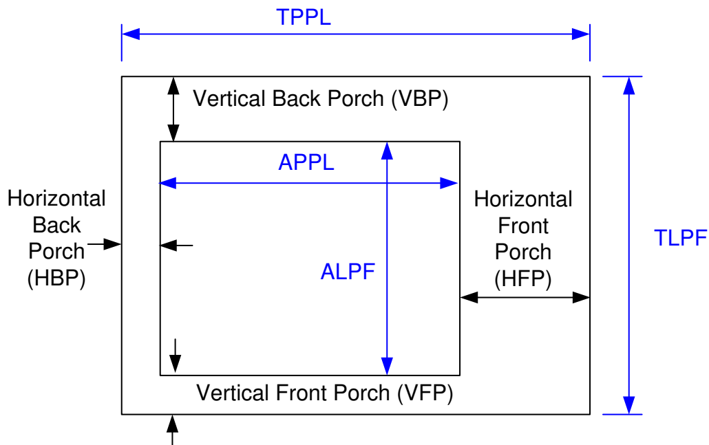
Figure 14. Video Timing Parameters
