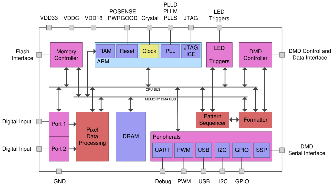
Figure 15. Functional Block Diagram
