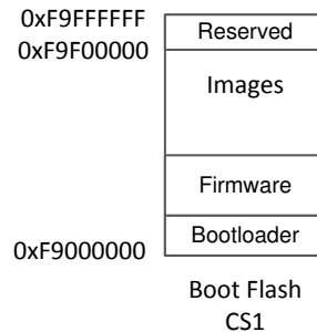
Figure 23. One 16-Mbit Flash Memory
