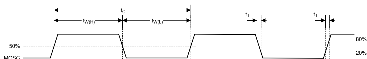
Figure 1. System Oscillators
