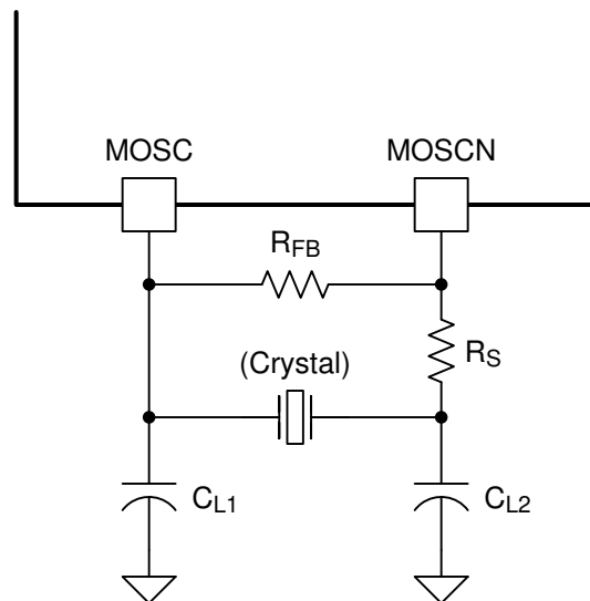
Figure 40. Crystal Oscillator Configuration
