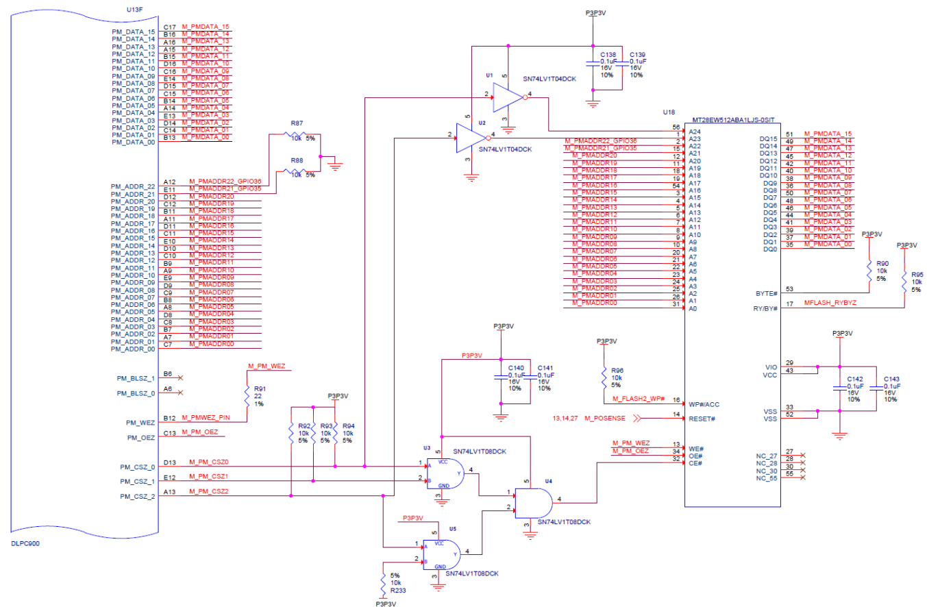
Figure 26. One 64-Mbit Flash Component
