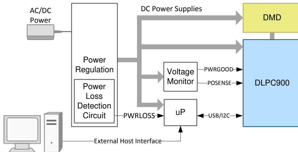
Figure 3. Power Distribution Layout Example
