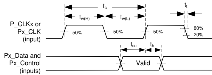
Figure 8. Input Port 1 and 2 Interface
