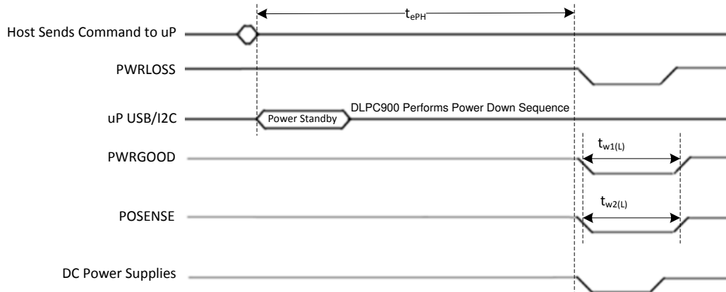
Figure 4. Anticipated Power Down Timing Diagram
