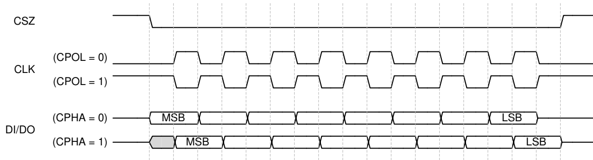
Figure 9. SSP Clock Mode Timing Diagram
