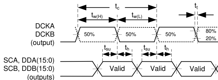
Figure 13. DMD LVDS Interface
