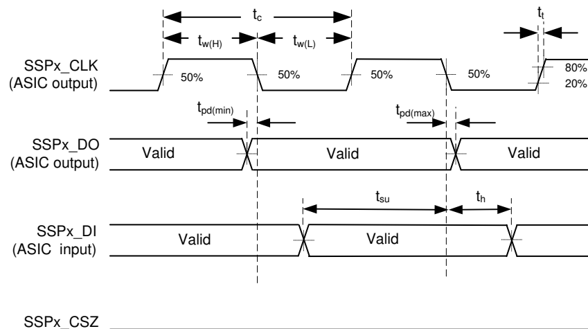
Figure 10. Synchronous Serial Port Interface – Master (Modes 0/3)
