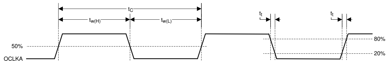
Figure 7. Programmable Output Clocks
