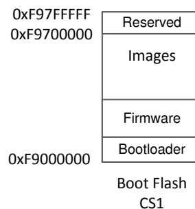
Figure 22. One 8-Mbit Flash Memory
