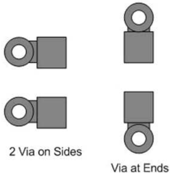
Figure 42. Decoupling Via Placement
