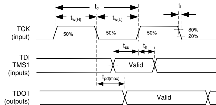
Figure 6. I/O Boundary Scan
