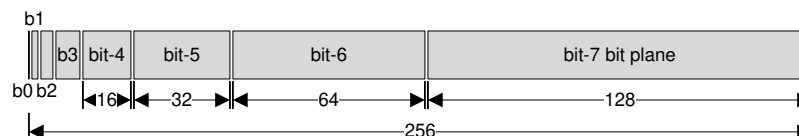
Figure 17. 24-Bit RGB Frame Bit Partition
