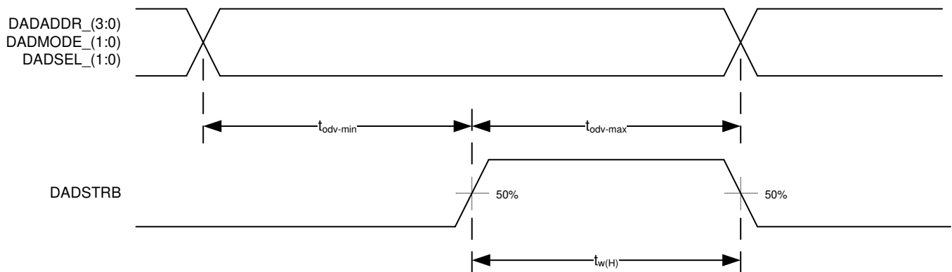
Figure 12. DMD Interface Timing
