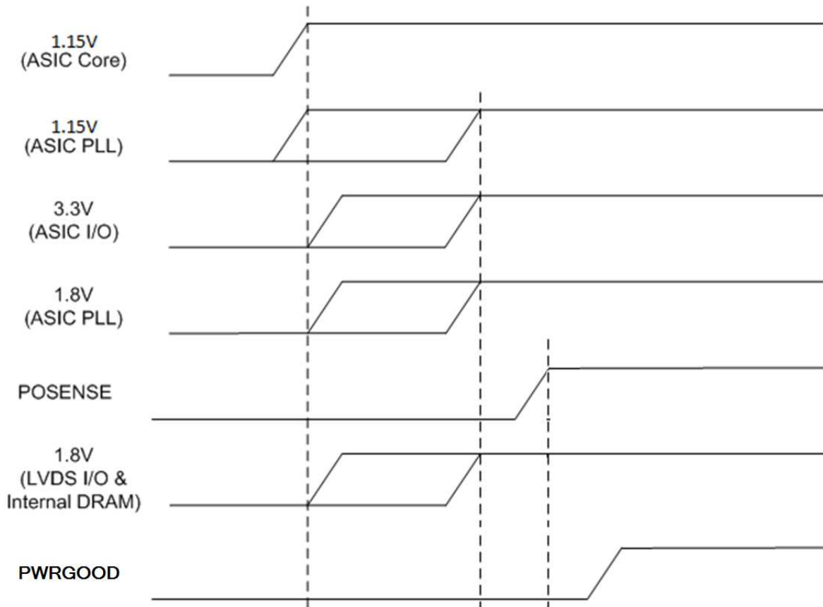
Figure 36. Power Sequencing
