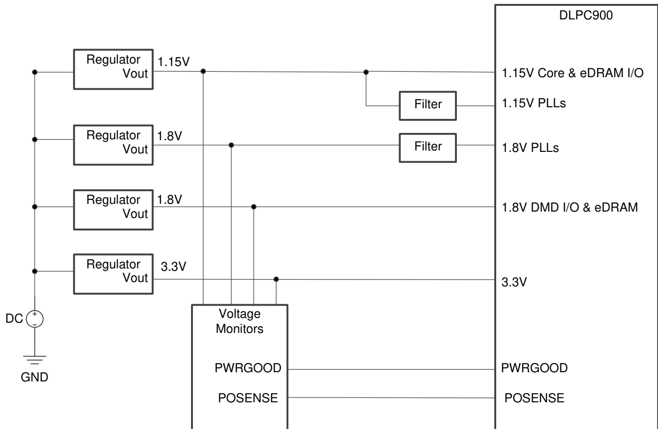
Figure 35. Power Regulation
