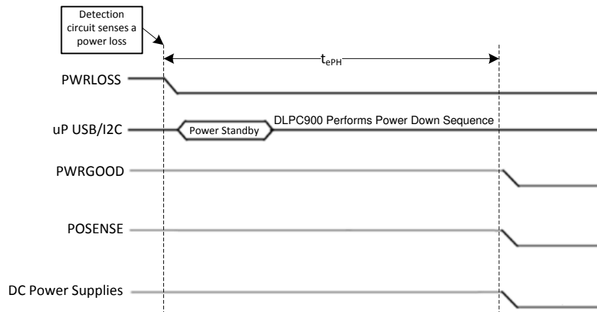
Figure 5. Unanticipated Power Loss Timing Diagram
