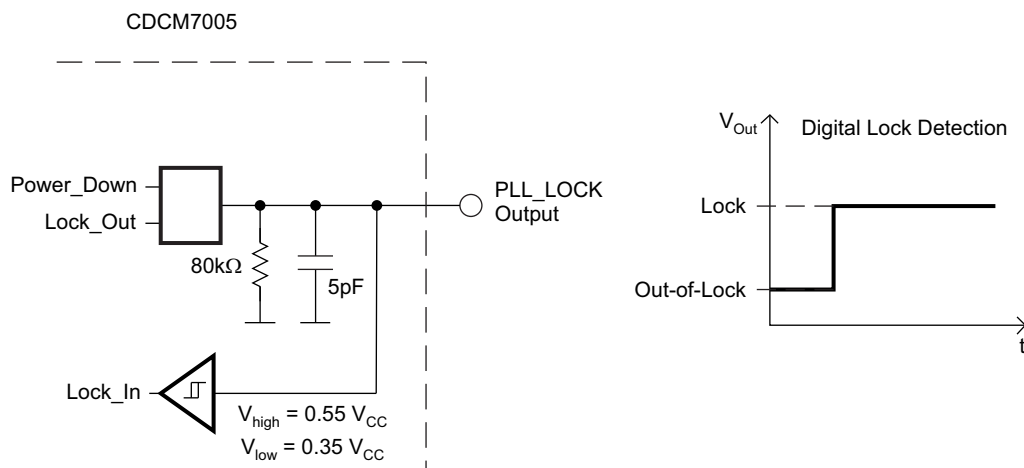
Figure 17. Digital Lock-Detect
