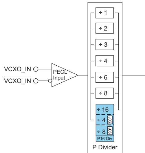
Figure 19. 90 Degree Phase Shift Option of P-Divider
