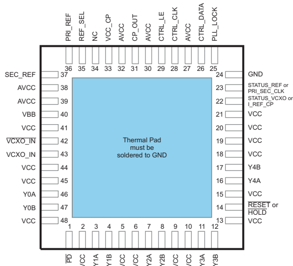
RGZ Package 48-Pin VQFN Top View
