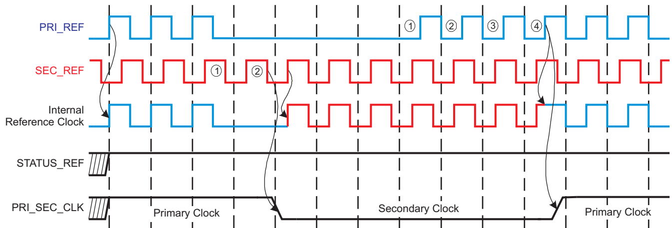
Figure 14. Behavior of STATUS_REF and PRI_SEC_CLK
