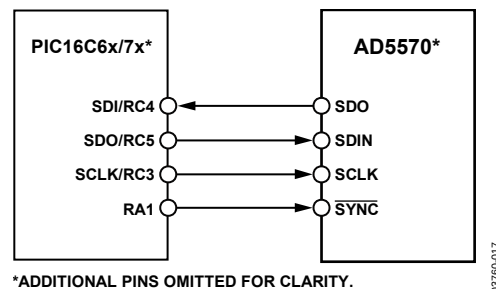
Figure 45. AD5570 to PIC16C6x/7x Interface
