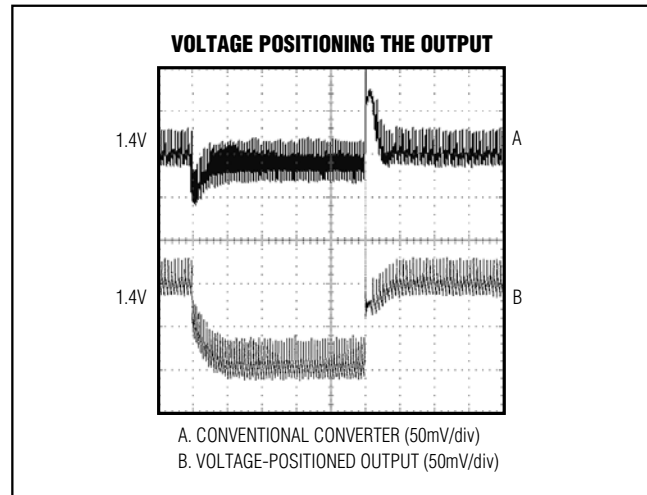
Figure 3. Voltage-Positioning and Nonvoltage-Positioning Waveforms
