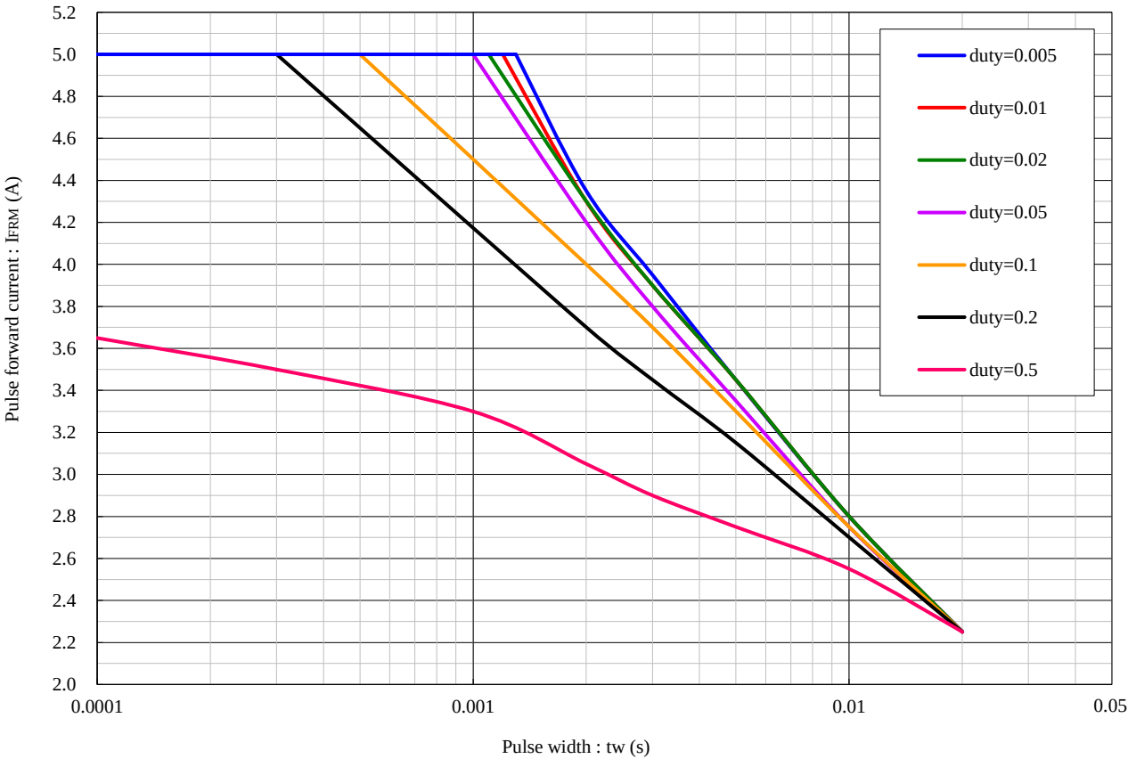
Maximum ratings of pulse forward current
