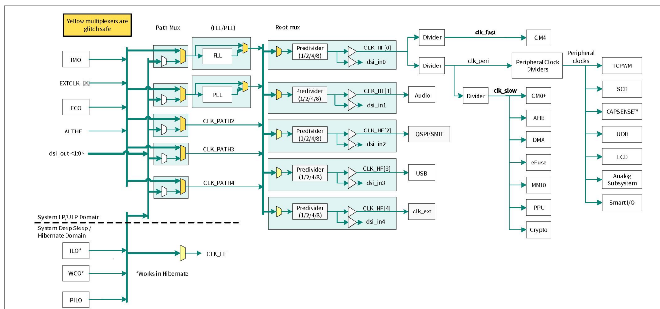
Figure 4 Clocking diagram
