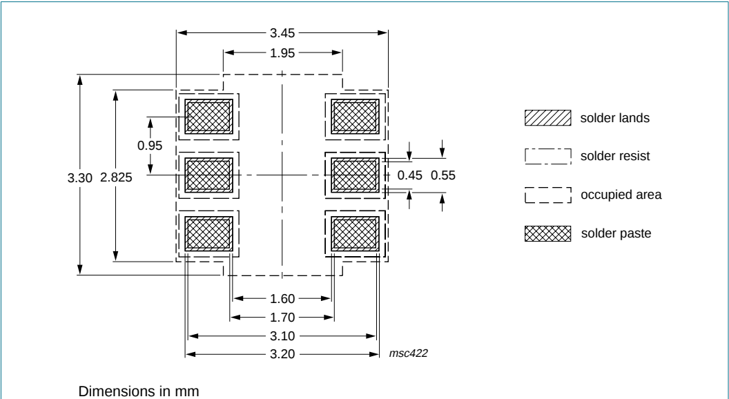
Fig 20. Reflow soldering footprint
