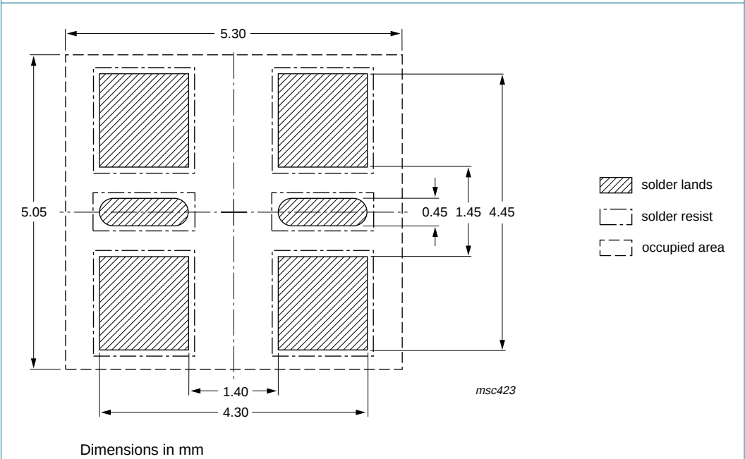
Fig 21. Wave soldering footprint
