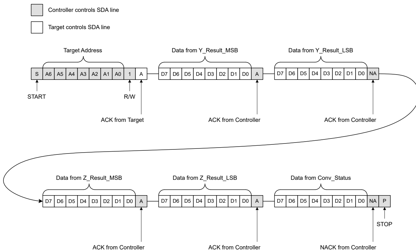
Figure 6-19. I 2 C Read Command for 16-Bit Data With CRC Disabled, Y and Z Axes Enabled
