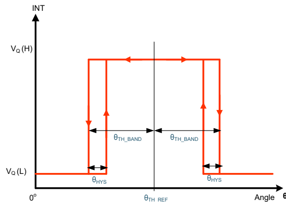
Figure 7-15. Angle Switch
