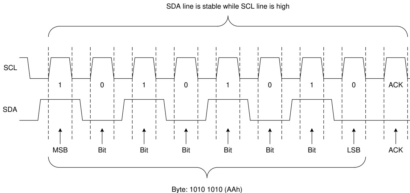
Figure 6-12. Bit Transfer
