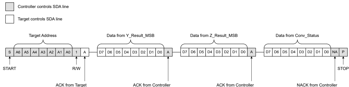
Figure 6-23. I 2 C Read Command for 8-Bit Data With CRC Disabled, Y and Z Axes Enabled
