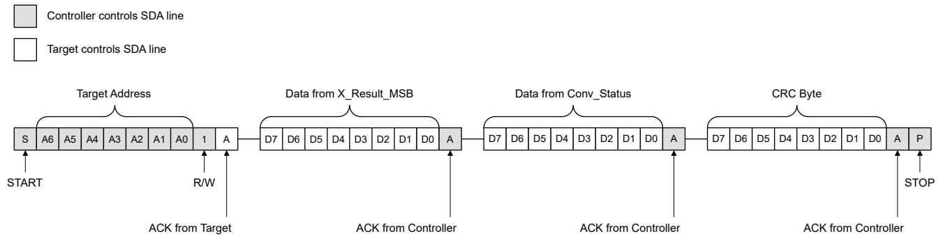
Figure 6-25. I²C Read Command for 8-Bit Data With CRC Enabled, X-Axis Enabled
