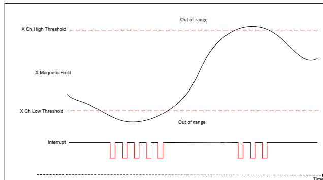
Figure 7-4. Magnetic Limit Cross Check With MAG_THR_DIR = 0h, THR_SEL[1:0] = 2h, INT_STATE = 1h
