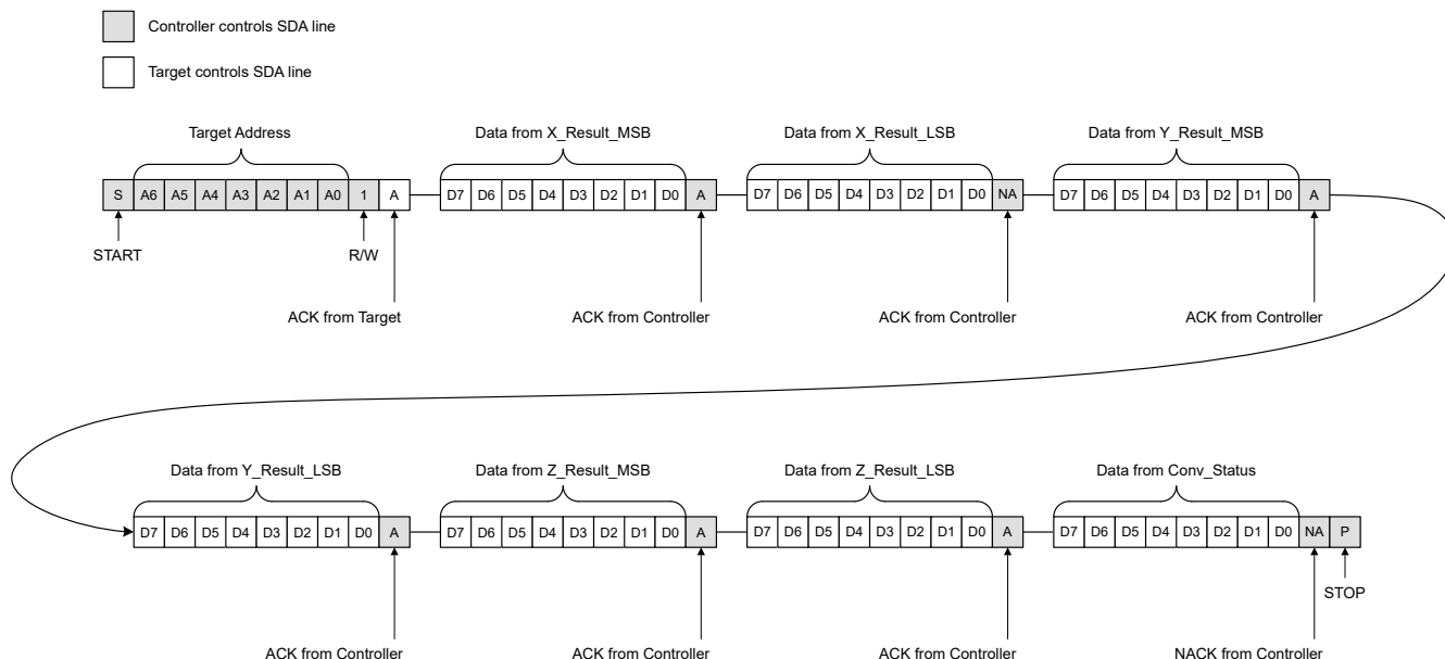
Figure 6-20. I²C Read Command for 16-Bit Data With CRC Disabled, X, Y, and Z Axes Enabled
