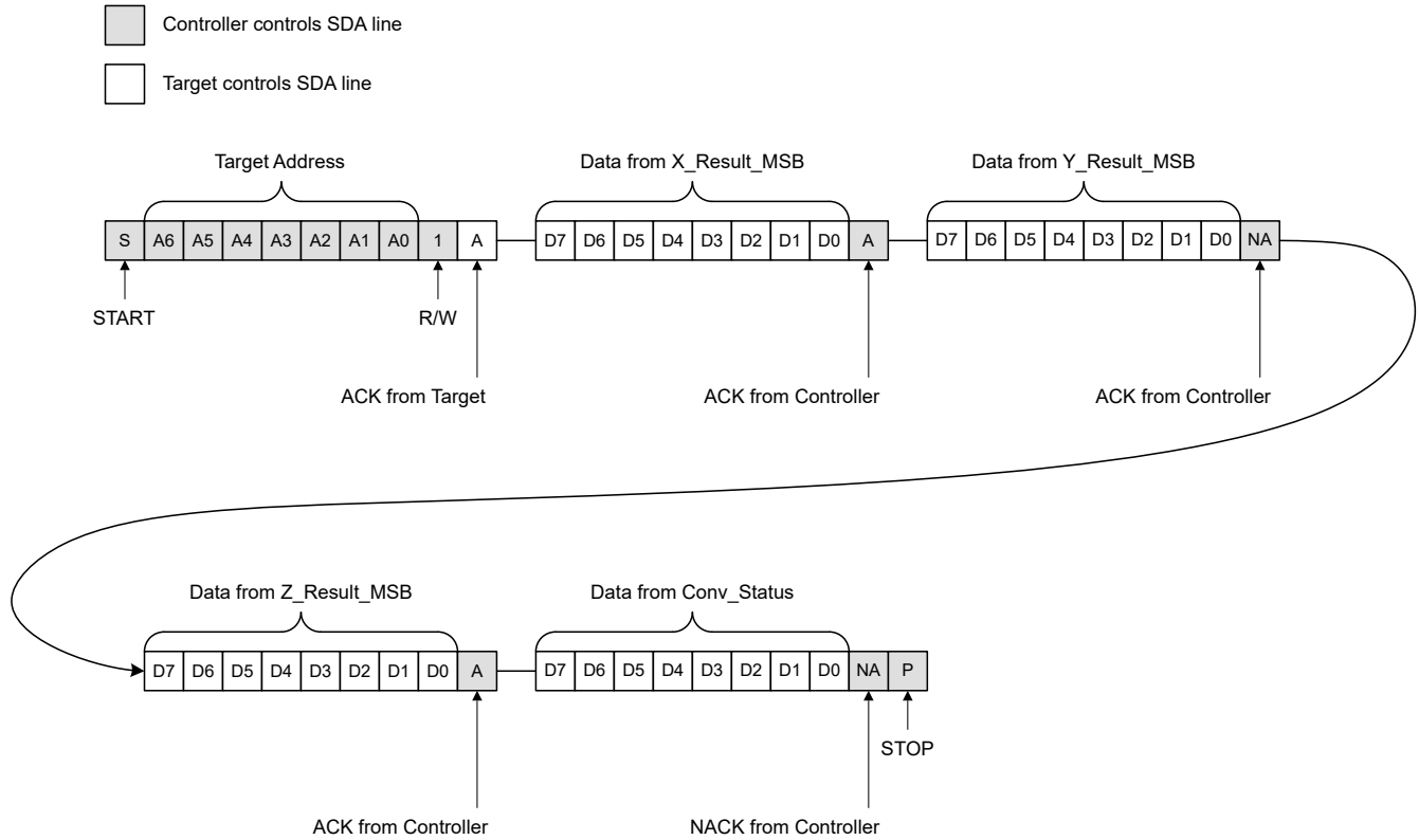
Figure 6-24. I²C Read Command for 8-Bit Data With CRC Disabled, X, Y, and Z Axes Enabled
