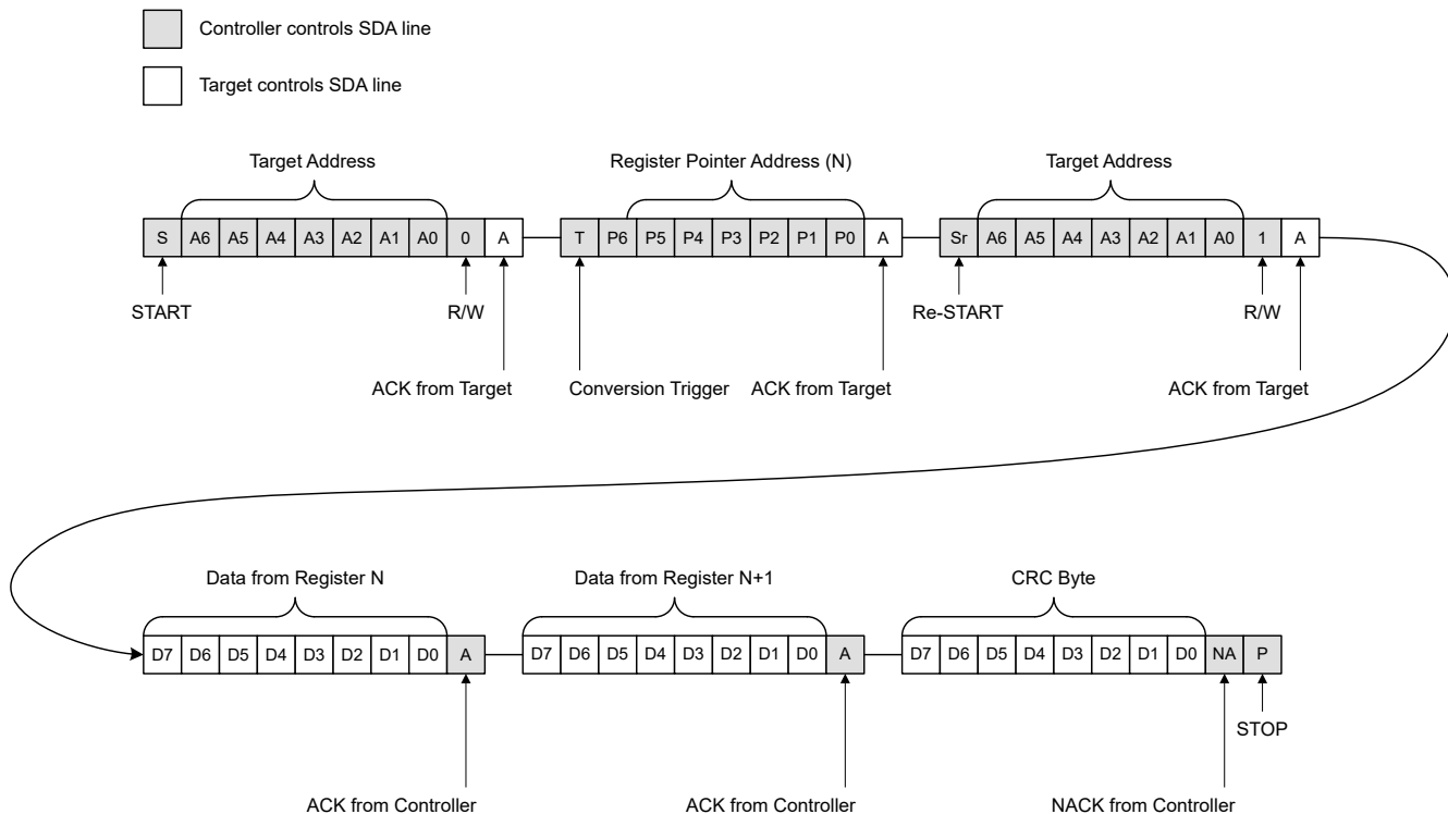
Figure 6-17. Standard I 2 C Read With CRC Enabled
