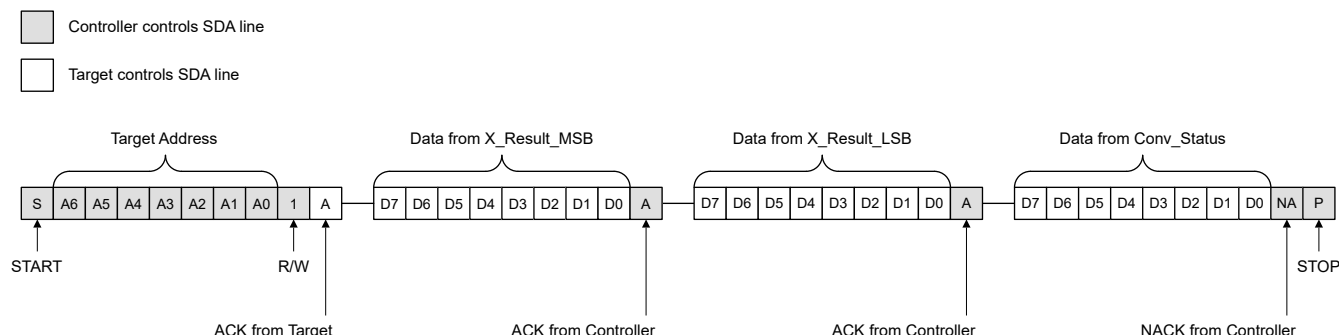
Figure 6-18. I 2 C Read Command for 16-bit Data With CRC Disabled, X-Axis Enabled
