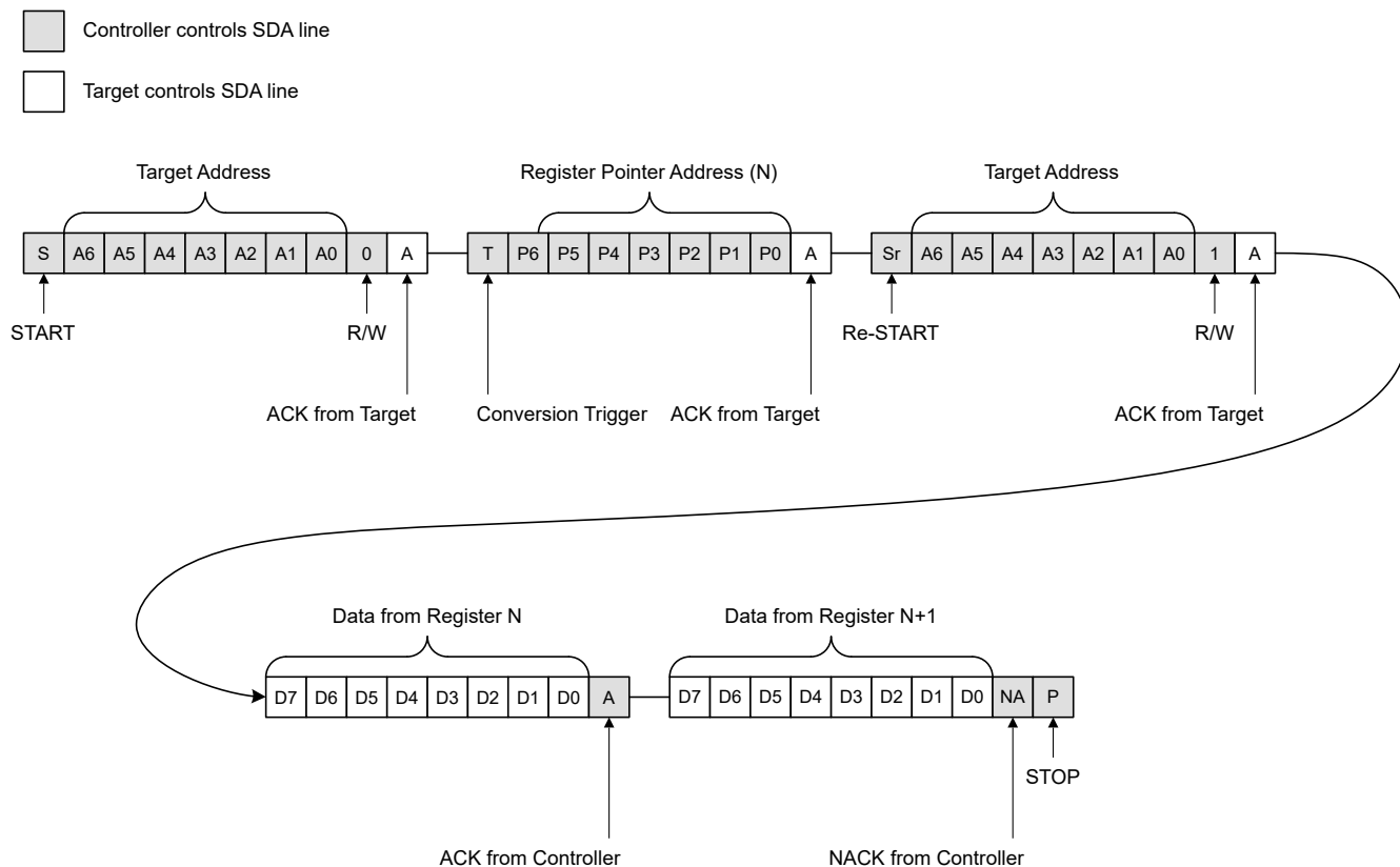
Figure 6-16. Standard I 2 C Read With CRC Disabled
