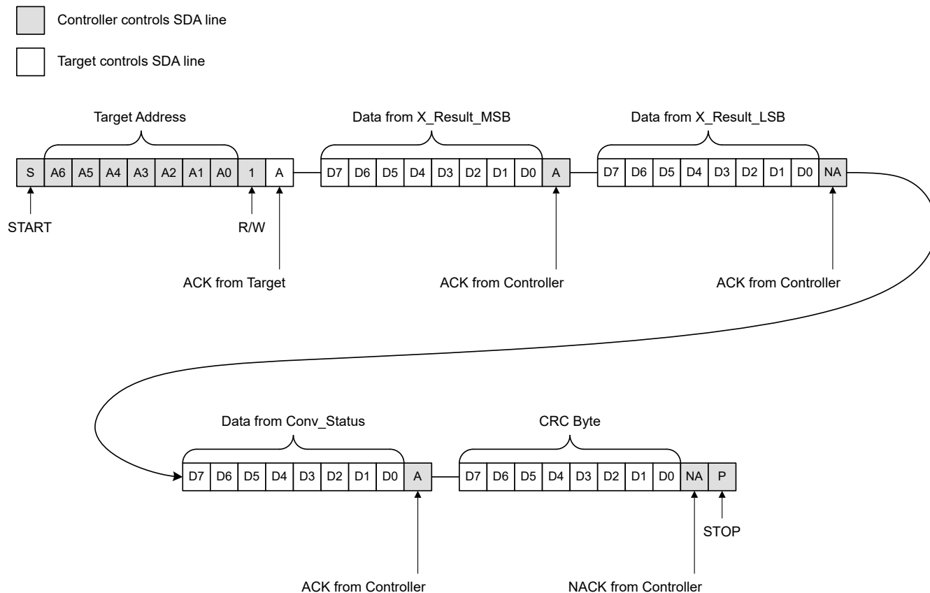
Figure 6-21. I²C Read Command for 16-Bit Data With CRC Enabled, X-Axis Enabled
