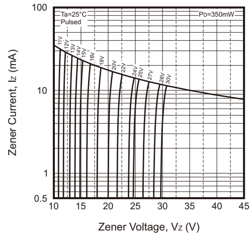
Fig.2 - Zener Characteristics
