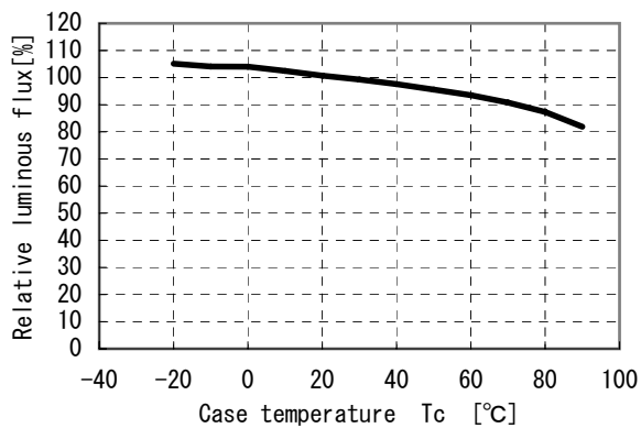
Relative luminous flux Vs Case temperature
